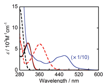
Fig. 1 UV-vis absorption spectra of \text{BIH} (black solid line), \text{BI}^+ (black broken line), \text{BI(OH)H} (red solid line), \text{BI(O}^{\cdot-})^+ (red broken line), and \text{Ru}_2\text{-Ru(CO)} (blue line, 1/10 intensity) in DMF-TEOA (4 : 1 v/v).
