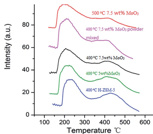
Fig. 6 \text{NH}_3 -temperature programmed desorption profiles of \text{MoO}_3/\text{H-ZSM-5} samples prepared via different conditions (impregnation/ powder mixing, 400\text{--}500\text{ }^\circ\text{C} ) together with the original H-ZSM-5 sample ( 400\text{ }^\circ\text{C} ).
