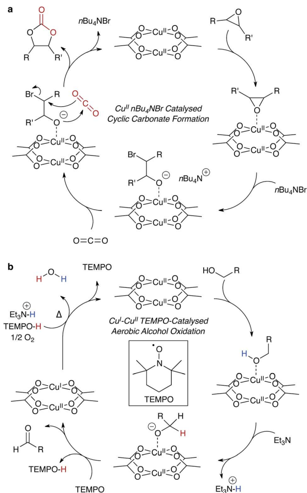
Fig. 5 An example of a heterogeneous catalytic cycle for the formation of cyclic carbonates – cupric acetate mediated – from epoxides and CO 2 . (a). n Bu 4 NBr serves as both a labile nucleophile and phase transfer reagent. The same cupric acetate motif may be used as a heterogeneous mixed redox Cu I /Cu II catalyst. (b), oxidising alcohols to aldehydes in the presence of TEMPO.
