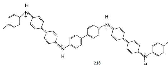
Fig. 182 Bipolaronic form of PDKA 218.
