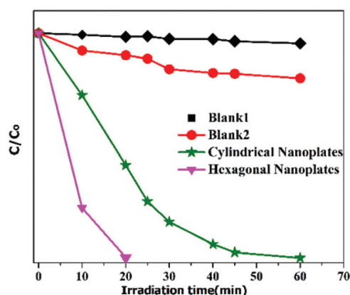
Fig. 6 Photodegradation of MB via two different \alpha - Fe_2O_3 nanoplates under visible-light illumination in the presence of H_2O_2 additive (blank 1: photodegradation of MB without additive under visible-light illumination, blank 2: photodegradation of MB under visible-light illumination in the presence of H_2O_2 only).
