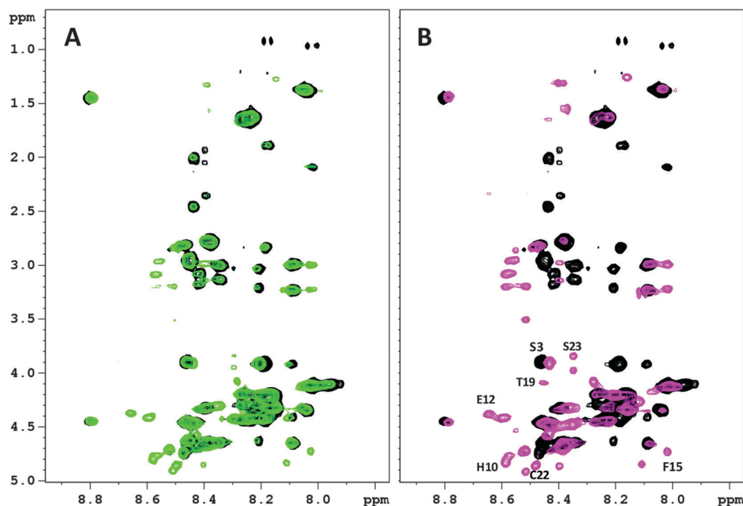
Fig. 8 2D ^1\text{H} - ^1\text{H} TOCSY spectra (NH-H \alpha region) of Bri2-23 0.5 mM in H _2\text{O} :D _2\text{O} 90:10 at 298 K and pH 3.0 in the presence of (A) 0.5 equivalents of Hg(II) ions; (B) 0.7 equivalents of Hg(II) ions.
