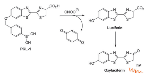
Fig. 81 Structure and reaction of luciferin based probe PCL-1 with ONOO - .
