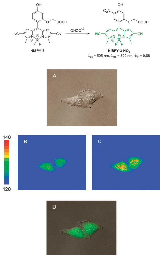
Fig. 79 Top: structure of NiSPY-3 and its reaction with ONOO - . Bottom: differential interference contrast (A), pseudo-colour fluorescence (B, C) and merged images (D) of HeLa cells loaded with NiSPY-3 . Pseudo-colour images were obtained before (B) and after (C) addition of peroxynitrite. Image reproduced with permission. 301
