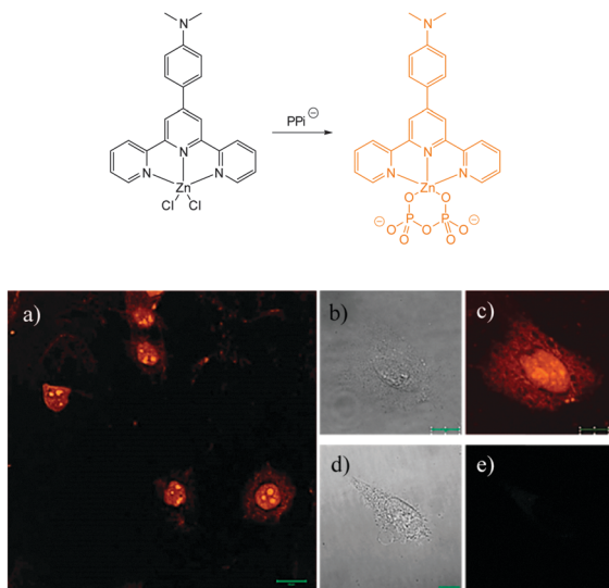
Fig. 44 Confocal fluorescence microscopy images of (a) HeLa cells incubated with probe 49 -ZnCl 2 (50 \mu M), (c) single HeLa cell, and (e) single HeLa cell without staining (control). Differential interference contrast images of (b) single HeLa cell incubated with probe 49 -ZnCl 2 (50 \mu M) and (d) single HeLa cell without staining (control). Image reproduced with permission. 195
