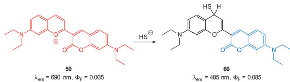
Fig. 53 Structure and reaction of 59 with HS^- .
