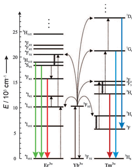
Fig. 1 Energy-level diagram of anti-Stokes processes in UCNPs ( \text{NaYF}_4 : \text{Yb} , \text{Er/Tm} ). The sensitizer ion \text{Yb}^{3+} absorbs NIR light, and the activator ions \text{Er}^{3+} or \text{Tm}^{3+} emit visible or NIR light. Sensitizer and activator ions are embedded in a hexagonal nanocrystal of \text{NaYF}_4 . Full arrows: radiative transitions, dotted arrows: non-radiative energy transfer, curled arrows: multiphonon relaxation. Adapted from ref. 2 with permission.
