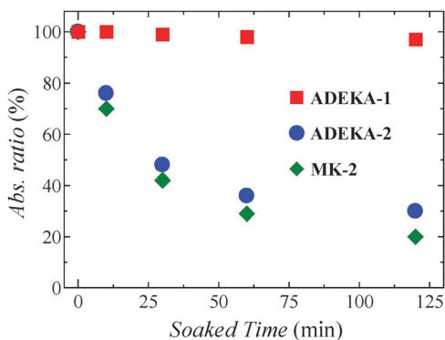
Fig. 2 Changes of the absorbances due to the carbazole dyes (ADEKA-1, ADEKA-2 and MK-2) adsorbed on the TiO 2 electrodes with the soaked time into 3-methoxypropionitrile–water (1:1 in volume) at 85 °C in the dark.
