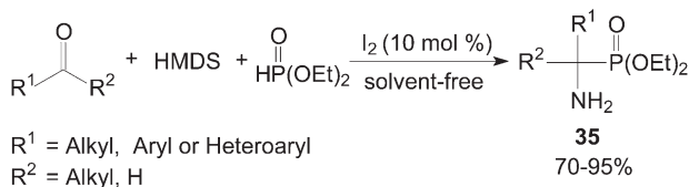
Scheme 18 Synthesis of the primary 1-aminophosphonate compounds.
