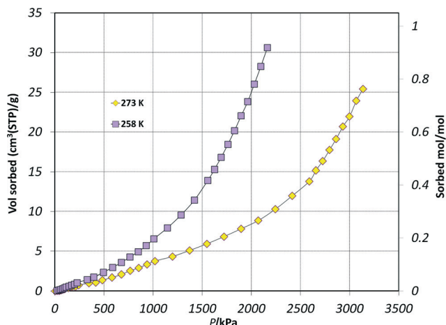
Fig. 3 \text{CO}_2 sorption isotherms of [\text{Cu}_2(\text{imdc})_2(\text{BF}_4)_2] ( 2 ) measured at 258 (purple squares) and 273 K (yellow diamonds) in [\text{Vol } \text{CO}_2 \text{ cm}^3(\text{STP}) \text{ per g}] and [\text{mol } (\text{CO}_2) \text{ per mol } [\text{Cu}_2(\text{imdc})_2](\text{BF}_4)_2] .
