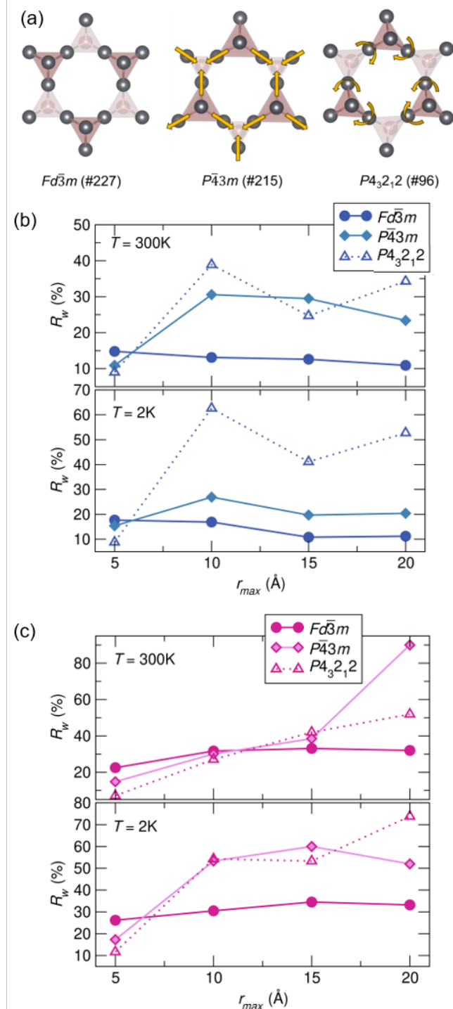
Fig. 5 (a) Distortions of the A-site cations in the various structural models. R_w as a function of box-car r_{max} for (b) \text{Bi}_{1.5}\text{Y}_{0.5}\text{Ti}_2\text{O}_7 at 300 and 2 K and (c) \text{Bi}_{1.5}\text{Ho}_{0.5}\text{Ti}_2\text{O}_7 at 300 and 2 K (NPDF, NOMAD, SNS).
