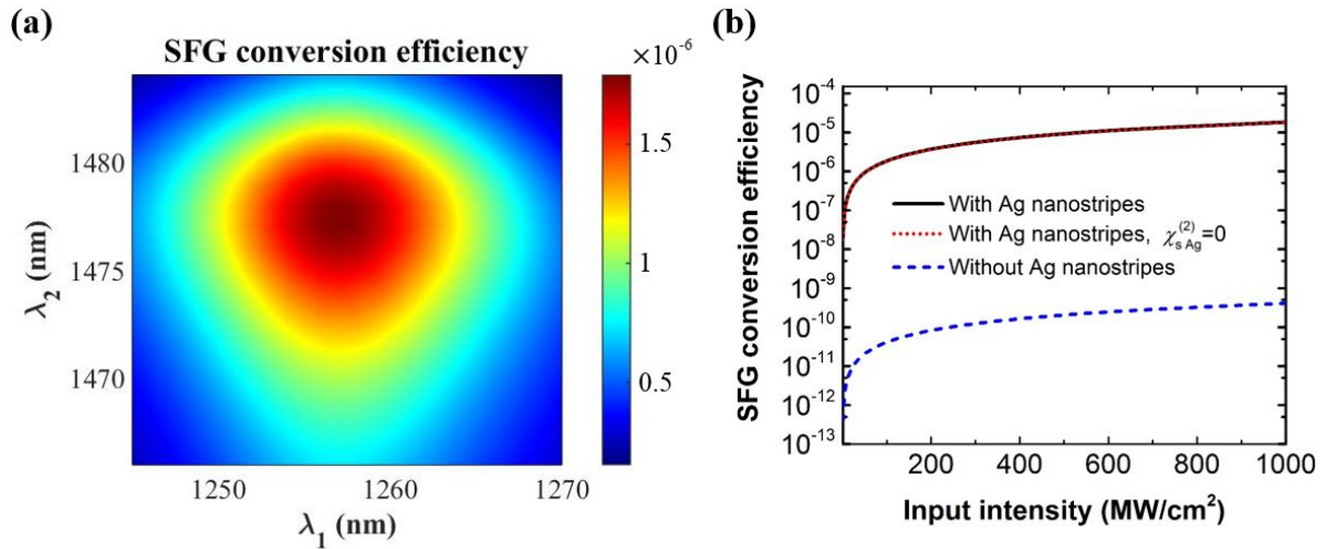
Fig. 3 (a) SFG conversion efficiency as a function of the two pump waves incident wavelengths.
