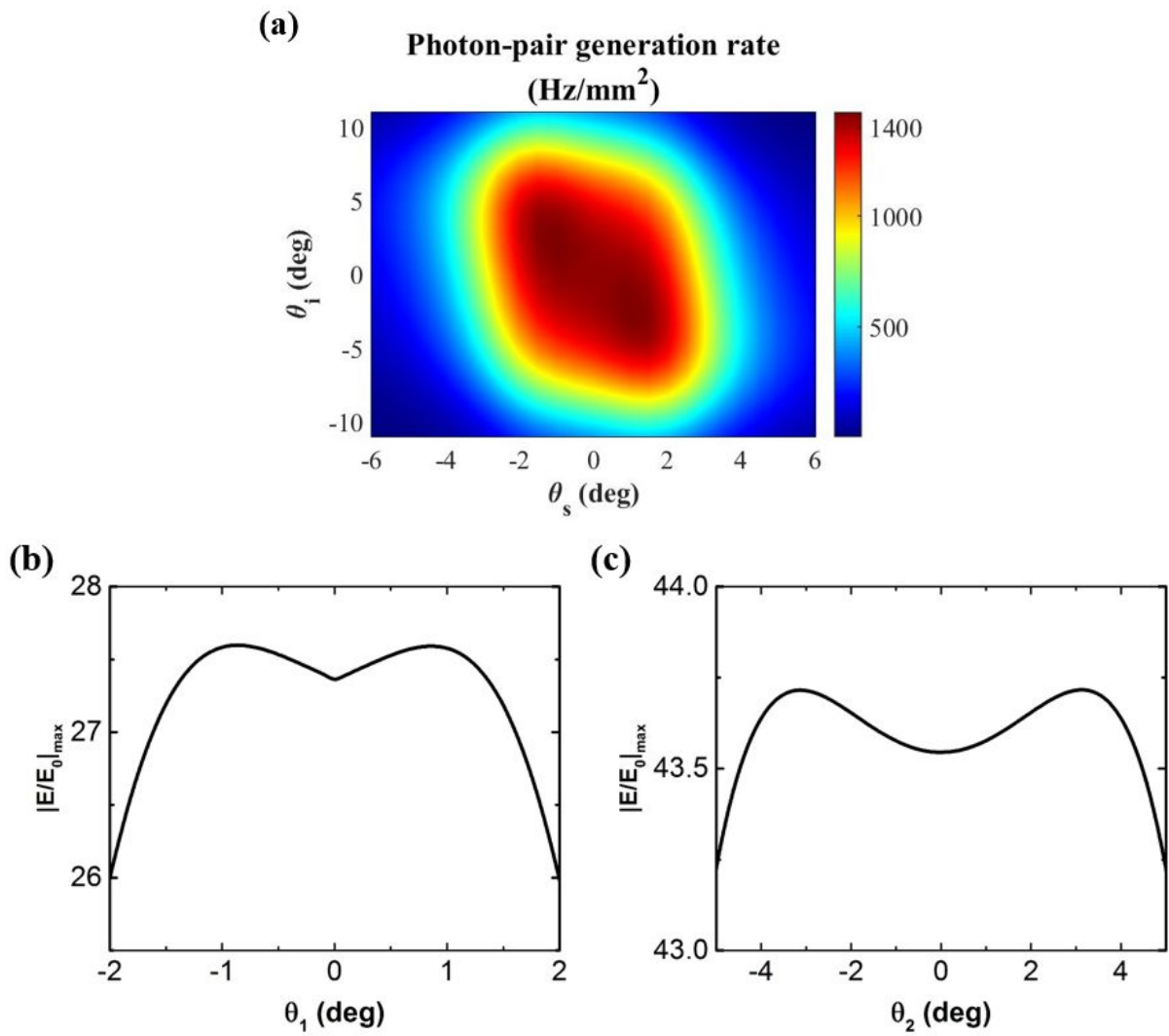
Fig. 7 (a) Photon-pair generation rate due to the boosted SPDC process as a function of the signal and idler wave observation angles ( \theta_s and \theta_i ). (b-c) The maximum electric field enhancement in the LiNbO 3 layer as a function of (b) \theta_1 and (c) \theta_2 in the classical counterpart of the SPDC process, i.e., SFG.
