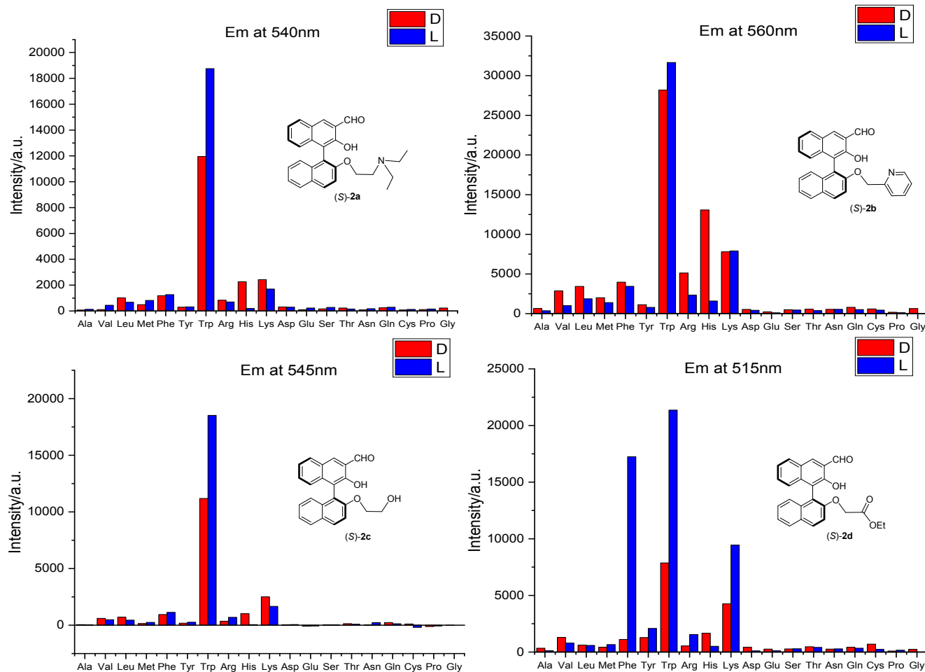
Figure 1. Fluorescence response of the micelle probes (S)-2a@PEG-PLLA, (S)-2b@PEG-PLLA, (S)-2c@PEG-PLLA and (S)-2d@PEG-PLLA towards various amino acids (Conditions: 10 \mu M micelle probe, 2 equiv \text{Zn}(\text{OAc})_2 , and 10 equiv amino acids in carbonate buffer solution. Peak intensities were used. Spectra were taken after 3 h of reaction at rt. \lambda_{\text{ex}} = 430 nm for (S)-2a, (S)-2b, and (S)-2c, and \lambda_{\text{ex}} = 400 nm for (S)-2d. slit = 3/3 nm, integration time = 0.1 s.)
