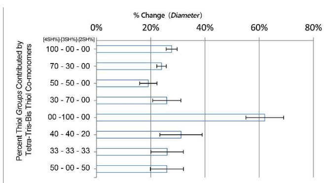
Figure 5. Swelling analysis of NIPU material mixtures. Compositions of thiol crosslinker of NIPU evaluated based on mixtures used, swelling in chloroform based on disk diameter changes. (4SH) = pentaerythritol tetrakis (3-mercaptopropionate), (3SH) = trimethylolpropane tris(3-mercaptopropionate), and (2SH) = 1,6-hexanedithiol. (n=3)
