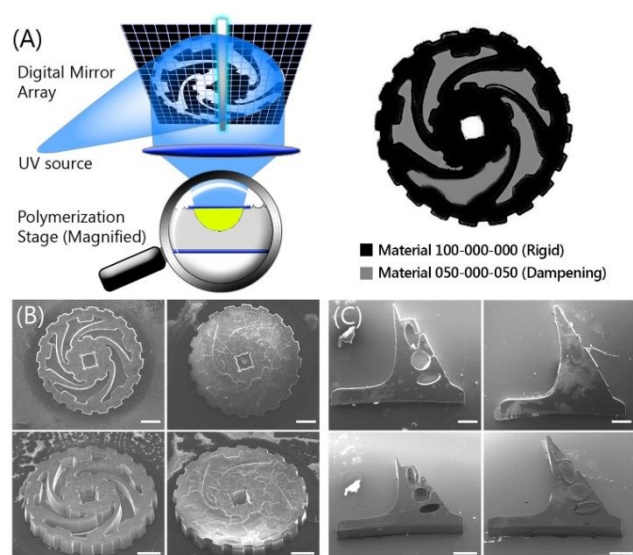
Figure 7. 3D printing of NIPU material: (A) schematic of the 3D projection printing setup with localization of printed materials. SEM images of printed NIPU structures; (B) A simple torque gear for dampening acceleration. (C) A pulsatile-flow cantilever valve. (B,C) Left images: More rigid material printed first. Right images: Compressible, damped, flexible, and elastic materials printed second. (Scale bar = 500 \mu m)
