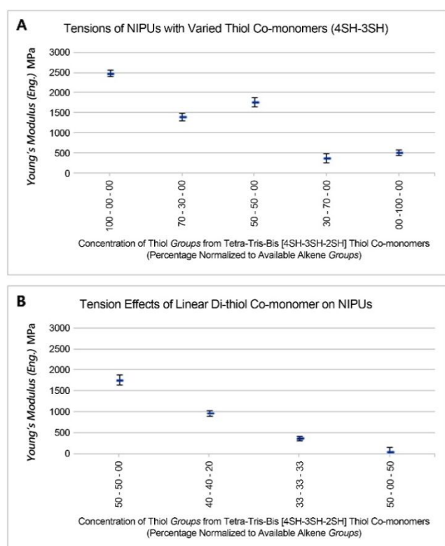
Figure 4. Tension testing for engineering Young's modulus. Compositions of thiol crosslinker of NIPU evaluated based on mixtures used were measured for elastic deformation. (4SH) = pentaerythritol tetrakis (3-mercaptopropionate), (3SH) = trimethylolpropane tris(3-mercaptopropionate), and (2SH) = 1,6-hexanedithiol. (n=5)
