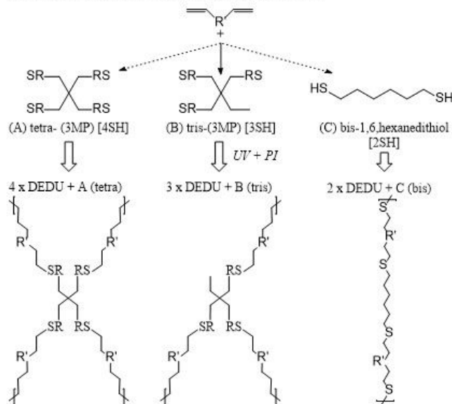
Figure 1. Schematic of the NIPU polymerization system. Synthesis of diallyl urethane prepolymer from diamine and TMPME-CC by heating, followed by UV-photoinitiated free radical thiol-ene polymerization with branched variable thiol crosslinkers, to create a 3D polymer network.
