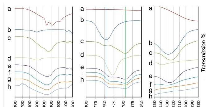
Figure 2. FTIR spectra of molecular precursors and products. (a) Cadaverine. (b) TMPMEC [5-allyloxyethyl-5-ethyl-1,3-dioxane-2-one (trimethylolpropane allyl ether-cyclic carbonate)]. (c) Product of heating cadaverine in the presence of TMPME-CC. Diallyl di-urethane (DEDU) product confirmed with replacement of cyclic-carbonate peaks with urethane (O=C-N) and hydroxyl (-OH) peaks. (d) Intermediate crosslinking thiol (3SH) = trimethylolpropane tris(3-mercaptopropionate). (e) Mixture of DEDU (c) and 3SH (d) exposed to 365 nm light for 0 min, (f) 2.5 min, (g) 5 min, and (h) 10 min. The peak at 927\text{cm}^{-1} , indicative of the alkene, diminishes with time and shows no difference between (g) and (h). Samples run in triplicate ( n=3 )
