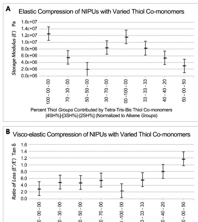
Figure 3. Compression testing by dynamic mechanical analysis. Compositions of thiol crosslinker of NIPU evaluated based on mixtures measured for (a) storage modulus and (b) ratio of loss \tan \delta . (4SH) = pentaerythritol tetrakis(3-mercaptopropionate), (3SH) = trimethylolpropane tris(3-mercaptopropionate), and (2SH) = 1,6-hexanedithiol. (n=3)
