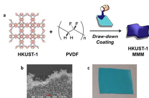
Fig 1. Schematic depicting the fabrication of mixed matrix membranes of HKUST-1. a. 3-Dimensional structure of HKUST-1, chemical structure of polyvinylidene difluoride, and schematic representing the MMM fabrication process, b. SEM image of HKUST-1 MMM c. Picture of HKUST-1 MMM.
