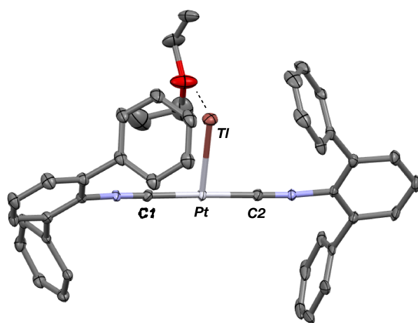
Figure 3. Molecular structure of [(Et 2 O)TI Pt(CNAr Dipp2 ) 2 ]BARF 4 ( 3 (Et 2 O)). Isopropyl groups and BARF 4 counterion have been omitted for clarity. The Pd congener 4 (Et 2 O) is isostructural.
