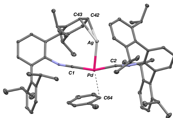
Figure 10. Molecular structure of [AgPd(CNR Dipp2 ) 2 ]( \eta^1 -C 7 H 8 )OTf ( 6 (C 7 H 8 )). Triflate counterion has been omitted for clarity.
