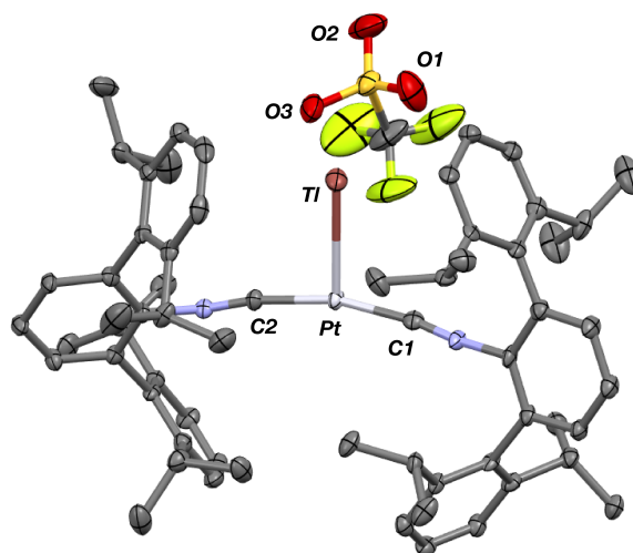
Figure 1. Molecular structure of [TIPt(CNAr Dipp2 ) 2 ] 2 OTf ( 1 ).
