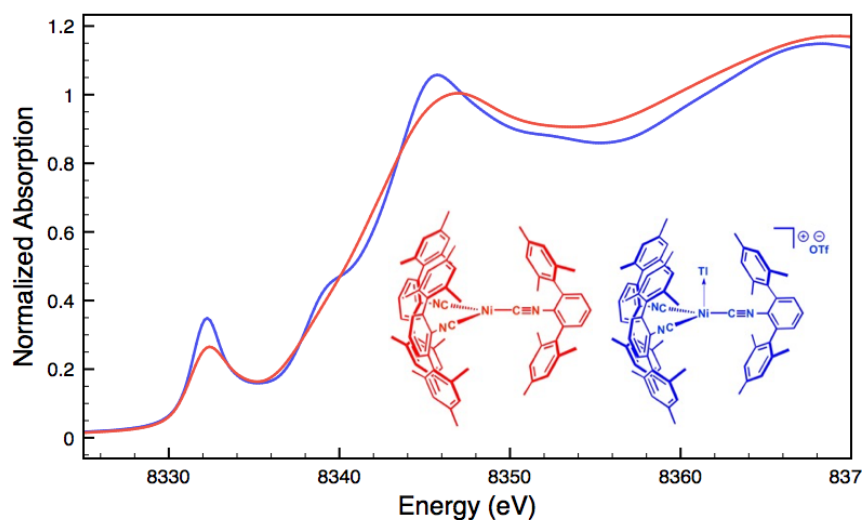
Figure 7. Comparative Ni K-edge XANES spectra of \text{Ni}(\text{CNAr}^{\text{Mes}2})_3 (red) and [\text{TlNi}(\text{CNAr}^{\text{Mes}2})_3]\text{OTf} (blue).
