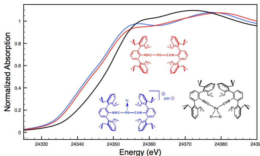
Figure 6. Comparative Pd K-edge XANES spectra of \text{Pd}(\text{CNAr}^{\text{Dipp}2})_2 (red), [\text{TlPd}(\text{CNAr}^{\text{Dipp}2})_2]\text{OTf} ( 2 , blue), and \text{Pd}(\eta^2\text{-O}_2)(\text{CNAr}^{\text{Dipp}2})_2 (black).
