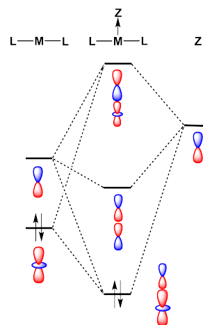
Figure 11. Molecular orbital diagram for a transition metal (M) bound to a \sigma -acceptor fragment (Z), showing how the LUMO of the resulting adduct can be stabilized with respect to the acceptor-free complex.
