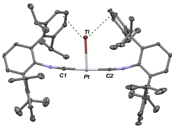
Figure 4. Molecular structure of [\text{TlPt}(\text{CNAr}^{\text{Dipp2}})_2]\text{BAR}^{\text{F}_4} ( 3 ). \text{BAR}^{\text{F}_4} counterion has been omitted for clarity.
