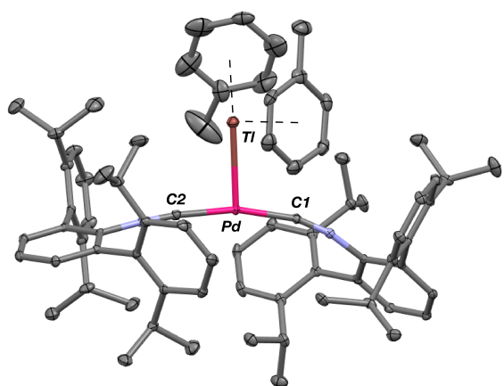
Figure 5. Molecular structure of [(\eta^6\text{-Tol})_2\text{TlPd}(\text{CNAr}^{\text{Dipp2}})_2]\text{BAR}^{\text{F}_4} ( 4(Tol)_2 ). \text{BAR}^{\text{F}_4} counterion has been omitted for clarity.
