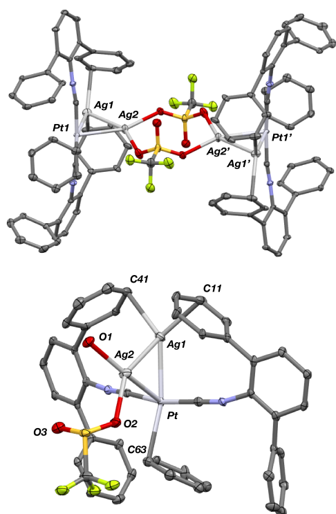
Figure 12. Molecular structure of the cationic portion of \{[Ag_2Pt(CNAr^{Dipp2})_2(\eta^1-C_6H_6)]_2(\mu-OTf)_2\}(OTf)_2 ( 7 ). Top: Full view of the centrosymmetric dication. Bottom: Truncated view of one triangulo - Ag_2Pt core. In both views, isopropyl groups and non-coordinating triflate anions have been removed for clarity.
