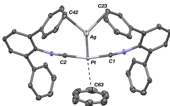
Figure 9. Molecular structure of [AgPt(CNR Dipp2 ) 2 ]( \eta^1 -C 6 H 6 )OTf ( 5 (C 6 H 6 )). Flanking isopropyl groups and the triflate counterion have been omitted for clarity.
