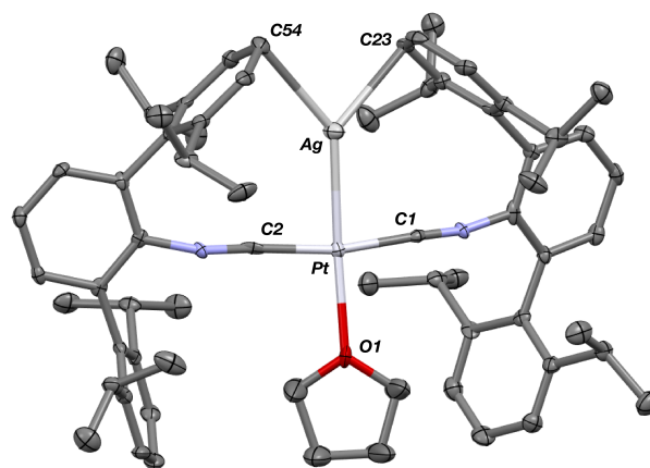
Figure 8. Molecular structure of [AgPt(CNR Dipp2 ) 2 ](THF)OTf ( 5 (THF)). The Pd congener 6 (THF) is isostructural. Triflate counterion has been omitted for clarity.
