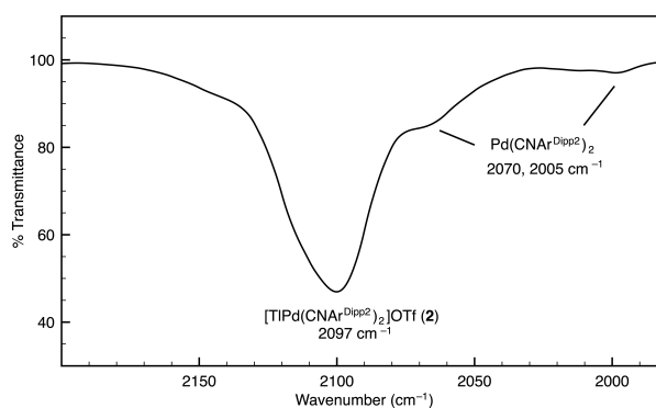
Figure 2. FTIR spectrum (ν(C≡N) region) of [TIPd(CNAr Dipp2 ) 2 ]OTf ( 2 ) showing the presence of Pd(CNAr Dipp2 ) 2 . Conditions: C 6 D 6 , 20 °C, KBr windows.
