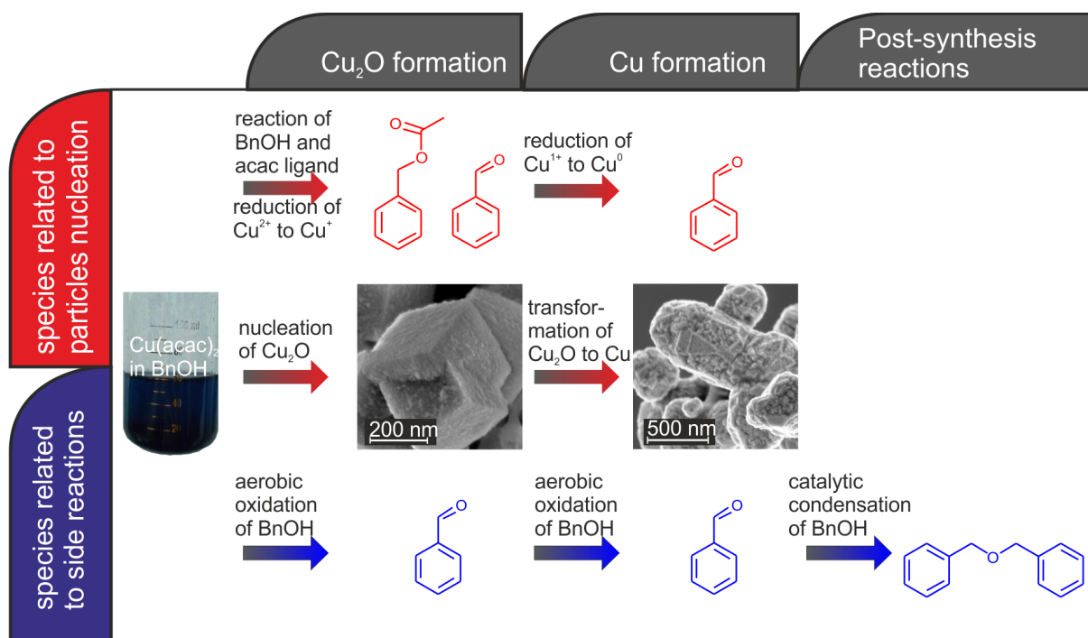
Figure 6 Overview on organic and inorganic reactions taking place during synthesis of copper nanoparticles.
