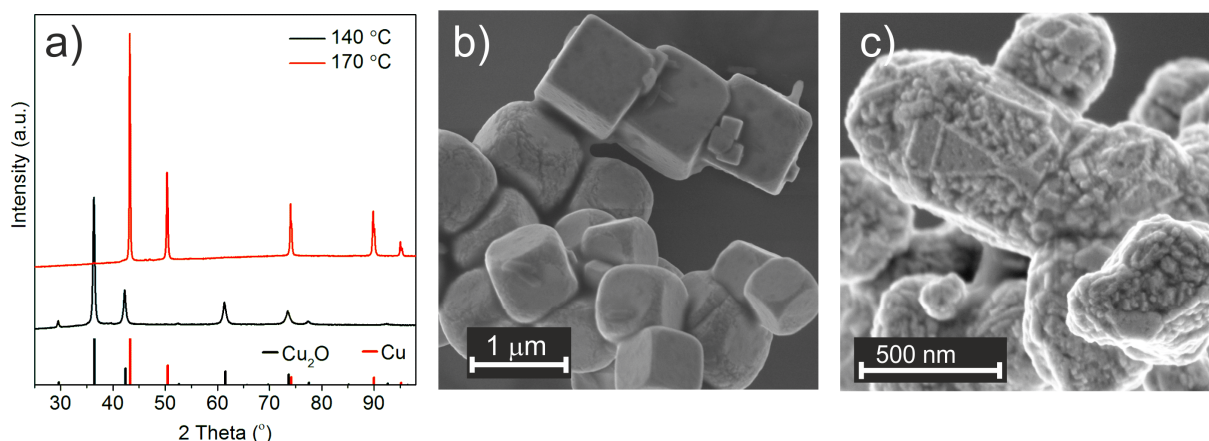
Figure 1 (a) PXRD patterns of the nanoparticles synthesized at 140 (black pattern) and 170 °C (red pattern). Reference XRD patterns of \text{Cu}_2\text{O} and Cu were simulated from International Center for Diffraction Data (ICDD) No. 00-005-0667 ( \text{Cu}_2\text{O} ) and ICDD No. 01-071-4610 (Cu). SEM images of (b) \text{Cu}_2\text{O} synthesized at 140 °C and (c) Cu synthesized at 170 °C.
