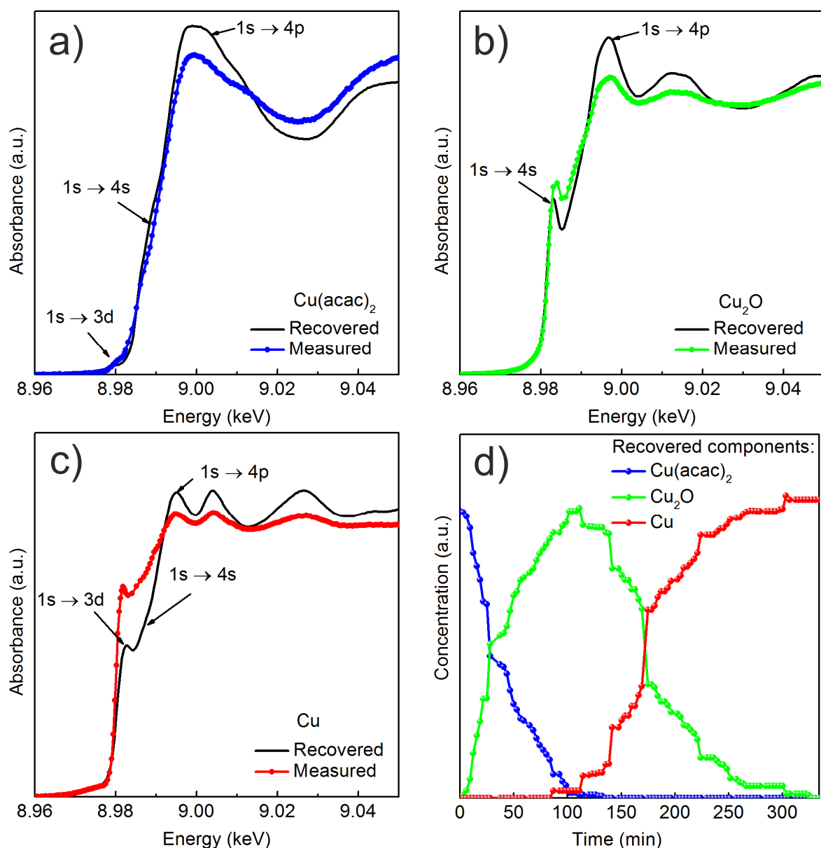
Figure 4 Results of the MCR-ALS analysis of in situ Cu K-Edge XANES spectra recorded in fluorescence mode; (a), (b) and (c) recovered spectra of individual components and corresponding reference spectra; The reference compounds were measured as pellets in transmission mode and are only given here as guidance; (d) concentration profiles of the three recovered components during the synthesis at 180^\circ\text{C} .
