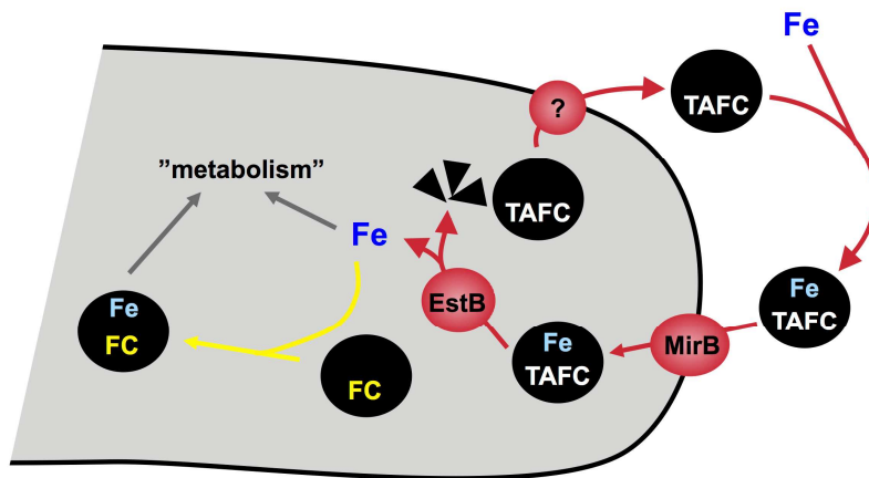
Fig. 2. Schematic view of TAFC-mediated iron acquisition and FC-mediated iron storage in A. fumigatus . The transporters for secretion of siderophores including TAFC (marked by a question mark) have not been identified yet.
