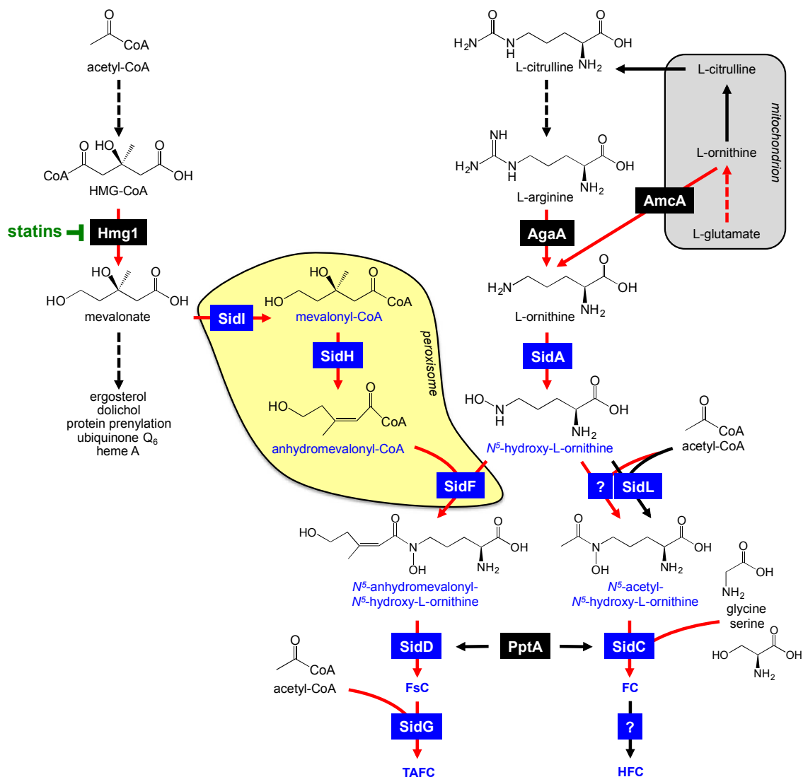
Fig. 3. A. fumigatus SB (in blue) and its links to the isoprenoid biosynthesis as well as ornithine/arginine metabolism. Involved enzymes are boxed and described in the text. Enzymatic steps transcriptionally upregulated during iron starvation are marked by red arrows. Broken arrows denote reactions involving more than one enzyme. Chemical structures of F s C, TAFC, FC and HFC are described in Fig. 1. Mitochondrion and peroxisome are shaded in grey and yellow, respectively.
