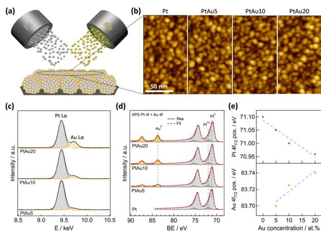
Fig. 1 (a) Illustration of the magnetron sputtering deposition process, (b) AFM images of the as-deposited pure Pt and Pt–Au alloy catalysts, (c) EDX and (d) XPS spectra acquired for the as-deposited Pt–Au alloy catalysts and pure Pt, and (e) Pt 4f 7/2 and Au 4f 7/2 peak positions extracted from the XPS spectra shown in (d).
