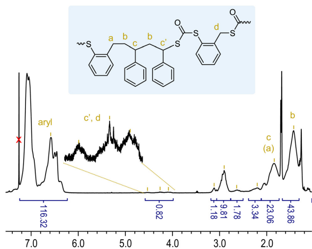
Fig. 6 ^1\text{H} NMR spectrum of \text{p}(\text{Sty}_{0.98}\text{-BOT}_{0.02})_n (Table 1, entry 9).
