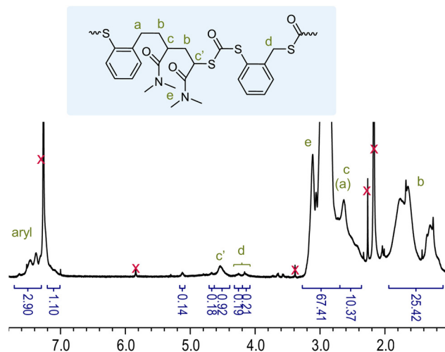
Fig. 2 ^1\text{H} NMR spectrum of \text{p(DMA}_{0.89}\text{-BOT}_{0.11})_n (Table 1, entry 5).
