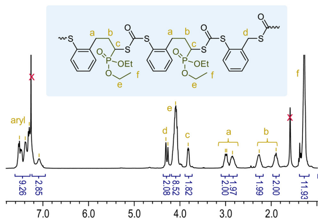
Fig. 5 ^1\text{H} NMR spectrum of \text{p}(\text{DEVP}_{0.4}\text{-BOT}_{0.6})_n (Table 1, entry 8).
