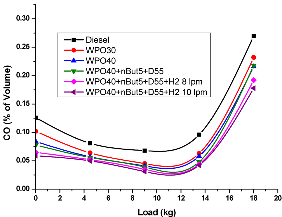
Fig. 7 Carbon monoxide emissions at different loads.
