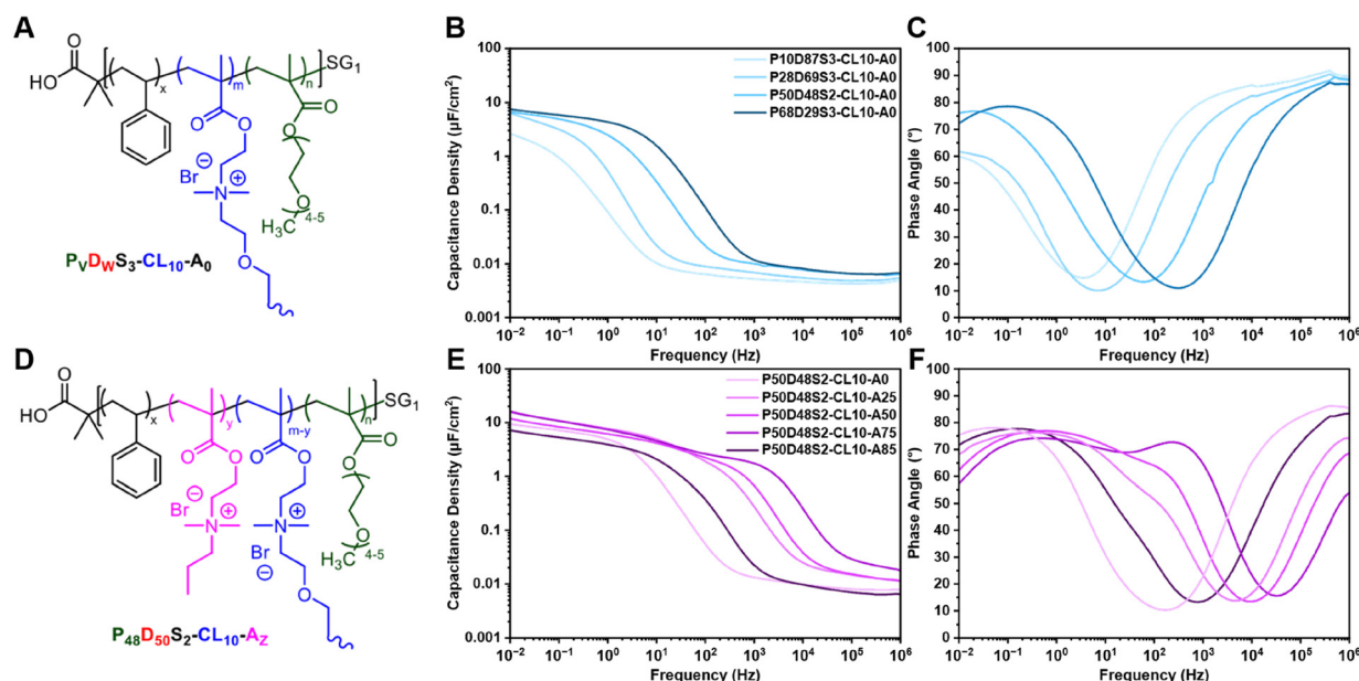
Fig. 3 Electrochemical impedance spectroscopy (EIS) results of the effect of changing mPEGMA to DMAEMA ratio in P_{VDW}S_X-CL_Y-CL_{10}-A_0 and effect of alkylation of P_{48D_{50}S_2-CL_{10}-A_Z} (A) chemical structure of P_{VDW}S_X-CL_Y-CL_{10}-A_0 , (B) capacitance density vs. frequency of mPEGMA to DMAEMA ratio in P_{VDW}S_X-CL_Y-CL_{10}-A_0 , (C) phase angle vs. frequency of mPEGMA to DMAEMA ratio in P_{VDW}S_X-CL_Y-CL_{10}-A_0 . The legend used in (B) is the same for (C). Results for P_{87D_{10}S_3-CL_{10}-A_0} was not included due to poor film formation. (D) chemical structure of P_{50D_{48}S_2-CL_{10}-A_Z} , (E) capacitance density vs. frequency of effect of alkylation of P_{50D_{48}S_2-CL_{10}-A_Z} , (F) phase angle vs. frequency of effect of alkylation of P_{50D_{48}S_2-CL_{10}-A_Z} . The legend used in (E) is the same for (F).
