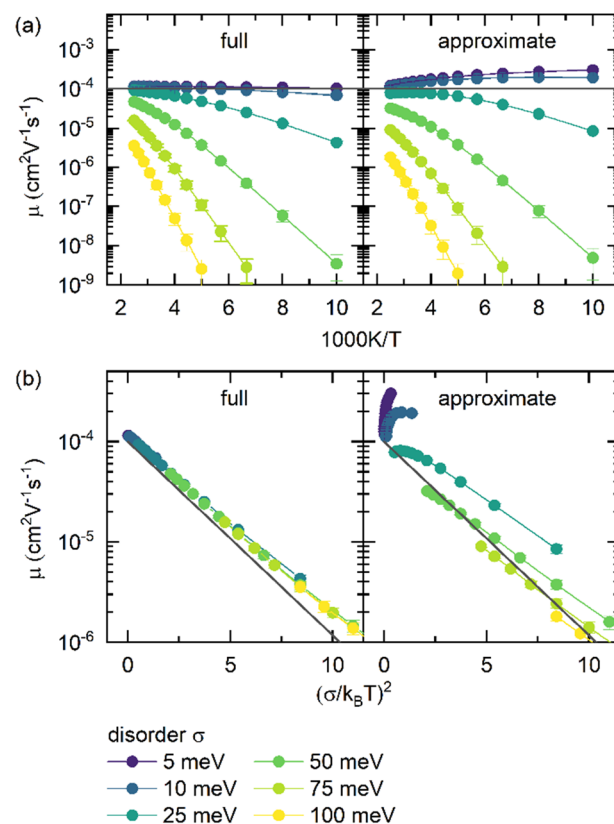
Fig. 3 Temperature dependence of the mobility for different \sigma = 5, 10, 25, 50, 75 , and 100 meV in an OLED-type device using either the full Miller–Abrahams hopping rate or the approximate expression. At high mobilities, the confidence intervals are smaller than the symbol size. (a) Results in an Arrhenius representation. The auxiliary line at 10^{-4} \text{ cm}^2 \text{V}^{-1} \text{s}^{-1} serves to differentiate the different temperature dependencies for 5 and 10 meV disorder for both rates. (b) Mobility plotted against the relative disorder (\sigma/k_B T)^2 . Beware that some data points pertaining to different values of \sigma coincide. The grey line shows an exponential decay with a decay constant of (2/3)^2 .
