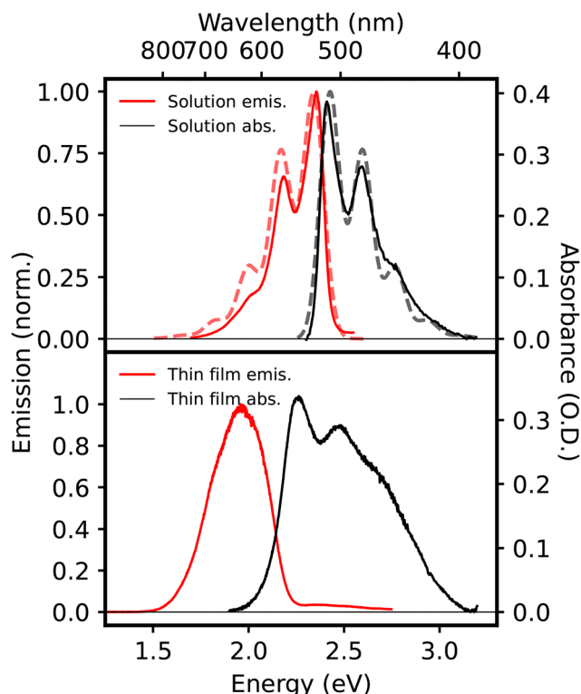
Fig. 2 Steady state spectroscopic characterisation of Red 254. UV-Vis absorption and emission spectra of a solution phase sample of Red 254 in DMSO (top) and absorption and emission spectra of sublimated thin films of Red 254 on a quartz-coated glass substrate (bottom). The emission spectra of both samples were taken with an excitation of 405 nm. The dashed line plots overlaid with the solution-phase spectra are Franck-Condon fits to the data, full details of which are displayed in the main body of text, as well as in Fig. S3 and S4 (ESI†) and in Table 2.
