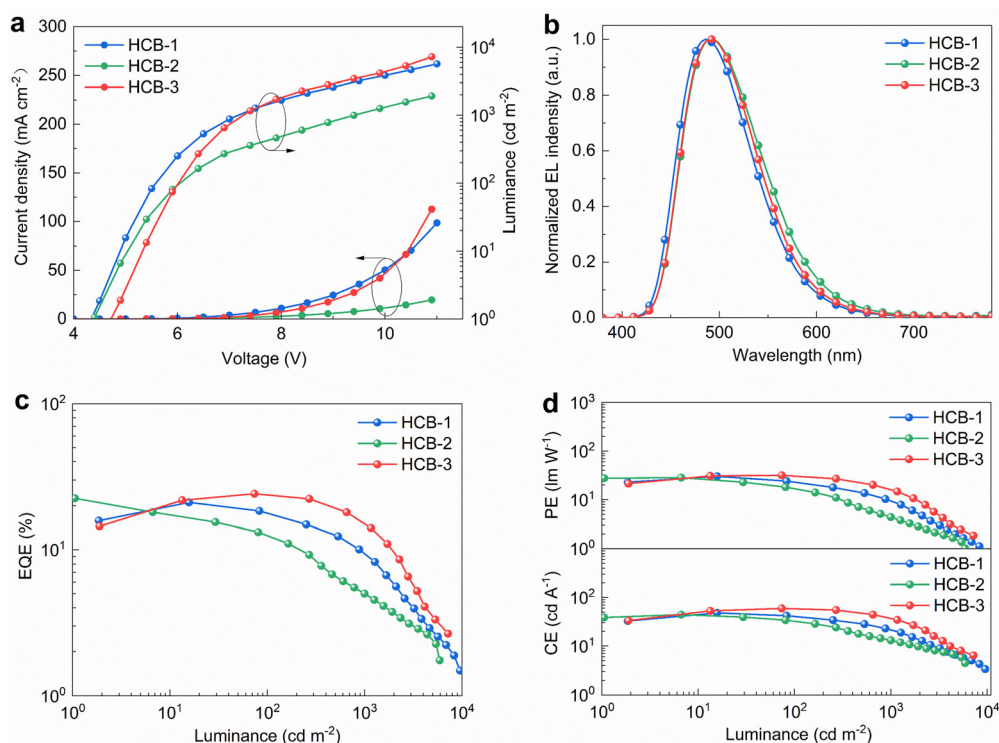
Fig. 5 (a) Current density and luminance versus voltage ( J - V - L ) characteristics. (b) EL spectra at a luminance of 1000 \text{cd m}^{-2} . (c) EQE as a function of luminance. (d) PE and CE as a function of luminance.
