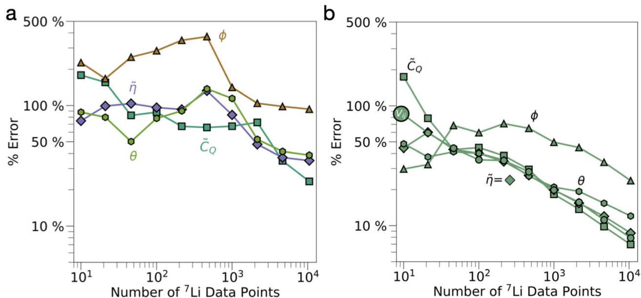
Fig. 5 Learning curves of the {}^7\text{Li} EFG performance metrics for scalar and tensorial learning approaches. (a) Learning curves for the four independent scalar learning models for \tilde{C}_Q , \tilde{\eta} , \theta , \phi shown in Fig. 3b. (b) Corresponding curves when extracting these quantities from the tensorial learning model in Fig. 3c. The line color corresponds to the model colors introduced in Fig. 3(b and c).
