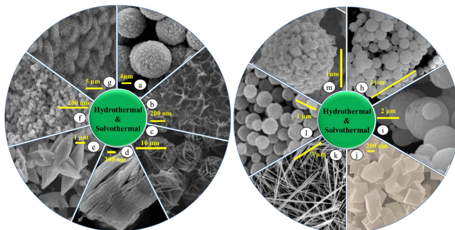
Fig. 3 ZMO morphologies produced by HT/ST synthesis (conditions for every morphology are reported in Table 1): (a) reproduced from ref. 72 with permission from Elsevier, copyright 2015, (b) reproduced from ref. 73 with permission from Elsevier, copyright 2022, (c) reproduced from ref. 74, (d) reproduced from ref. 75 with permission from Elsevier, copyright 2020, (e) reproduced from ref. 76 with permission from Elsevier, copyright 2021, (f) reproduced from ref. 70 with permission from Elsevier, copyright 2018, (g) reproduced from ref. 55 with permission from Elsevier, copyright 2018, (h) reproduced from ref. 77 with permission from Wiley Online Library, copyright 2022, (i) reproduced from ref. 78 with permission from Elsevier, copyright 2021, (j) reproduced from ref. 79 with permission from Elsevier, copyright 2019, (k) reproduced from ref. 53 with permission from Elsevier, copyright 2015, (l) reproduced from ref. 39 with permission from ACS, copyright 2018, and (m) reproduced from ref. 65 with permission from Elsevier, copyright 2014.
