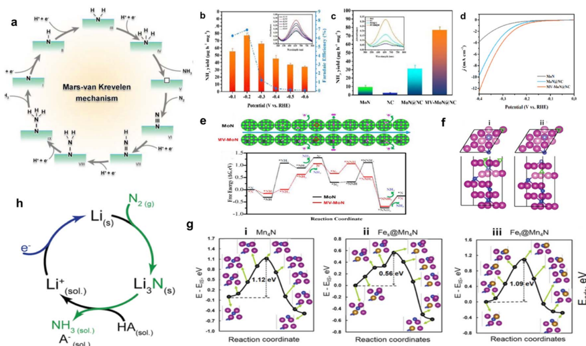
Fig. 30 (a) Schematic of the Mars van Krevelen mechanism for NRR. Adapted with permission from ref. 219. Copyright 2023, John Wiley and Sons. (b) Variation of NH 3 yield rates and faradaic efficiency (blue dashed line) with the potential for MV-MoN@NC. (c) Ammonia yield at -0.2 V vs. RHE for different catalysts used in the study. (d) Polarization curves for MoN, MoN@NC and MV-MoN@NC. (e) Gibbs free energy evolved for nitrogen reduction reactions at different reaction coordinates for MoN and MV-MoN. Adapted with permission from ref. 220. Copyright 2020, Elsevier. (f) Sublayer lattice nitrogen diffusion during (i) initial stage and (ii) final stage (downward green triangle: surface N vacancy; upward green triangle: sublayer N vacancy; magenta: Mn atoms; blue: N atoms). (g) Potential energy surfaces for the diffusion of nitrogen onto the surface from the sublayer (magenta: Mn; gold: Fe; green: Ni; blue: N). Adapted with permission from ref. 221. Copyright 2018, American Chemical Society. (h) Schematic representation of the mechanism of lithium-mediated ammonia synthesis. Adapted from the work of Krishnamurthy et al. , 222 licensed under CC-BY-NC-ND 4.0 ( https://creativecommons.org/licenses/by-nc-nd/4.0/ )/cropped from original.
