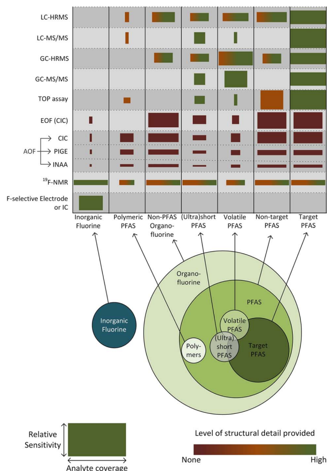
Fig. 3 Outline of the analytical techniques that may be applied to close the fluorine mass balance in PFAS. The widths of the boxes show the general coverage of the technique within the appropriate category of fluorinated chemicals, and the heights indicate the general sensitivity of the method. Reproduced from ref. 56 Copyright 2024, ACS.
