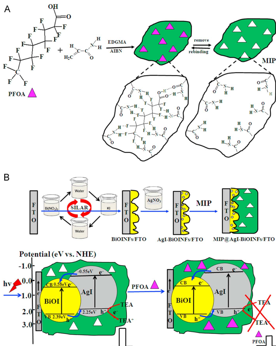
Fig. 11 A) Schematic of molecularly imprinted polymer (MIP) formation. (B) Schematic of the SILAR deposition of AgI-BiOINf films on MIP and the principle of PFOA PEC determination utilizing MIP@AgI-BiOINfs/FTO. Reproduced from ref. 101 Copyright 2015, Elsevier.
