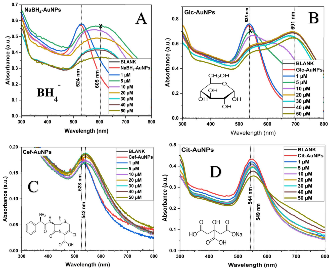
Fig. 1 UV-vis Spectroscopy of AuNPs interacting with mercury at different concentrations showing the absorption patterns of (A) NaBH 4 -reduced AuNPs, (B) Glc-AuNPs, (C) Cef-AuNPs, and (D) Cit-AuNPs.
