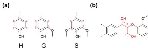
Fig. 1 Chemical structures of (a) the aromatic units found in lignin and (b) the main linker group present in lignin, β-O-4 (red).
