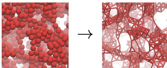
Figure 1. Schematic view of the particles' and bonds' representation within each cluster or connected component, to be used for the purpose of network quantification.
