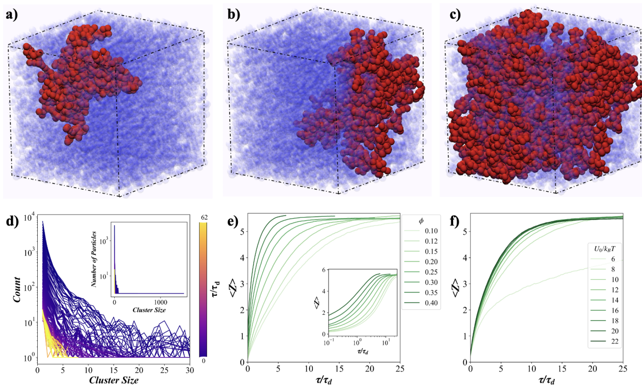
Figure 3. (a-c) Three different snapshots of the largest connected component within the system during gelation at times ( \tau/\tau_d ) 1.3, 1.4, and 1.5, respectively, for a system with \phi = 0.2 and an attraction strength of U_0 = 20k_B T . (d) Cluster size distribution during gelation, excluding the largest cluster for the same system. The cluster size represents the number of colloidal particles within each individual cluster. Changes in the ensemble-averaged coordination number, \langle Z \rangle , during gelation for: (e) different volume fractions at an attraction strength of U_0 = 20k_B T , and (f) different attraction strengths at the volume fractions of \phi = 0.2 .
