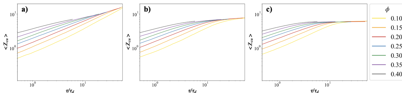
Figure 8. Ensemble-averaged unique coordination number, Z_{cu} , versus gelation time (scaled by the particle diffusion time) for different volume fractions at the same attraction strength of: (a) U_0 = 6k_B T , (b) U_0 = 8k_B T , and (c) U_0 = 20k_B T .
