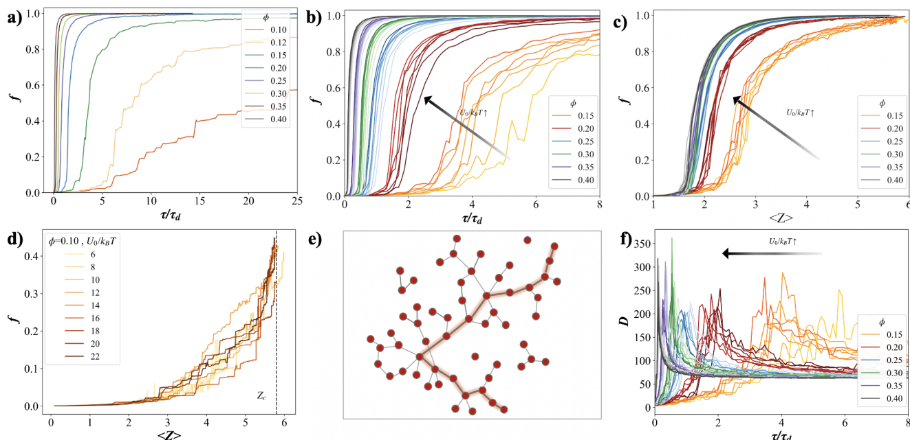
Figure 4. Fraction of total particles in the largest cluster for: (a) all volume fractions and the attraction strength of U_0 = 20k_B T versus gelation time; (b) and (c) volume fraction of \phi \geq 0.15 and all attraction strength, plotted versus gelation time and versus the ensemble-averaged coordination number, \langle Z \rangle , respectively; (d) volume fraction \phi = 0.1 and all attraction strength. (e) Schematic illustrating the diameter of a particle network, defined as the longest among all shortest paths between pairs of particles. The highlighted line marks the two particles connected by this path. (f) Network diameter versus gelation time for systems with \phi \geq 0.15 .
