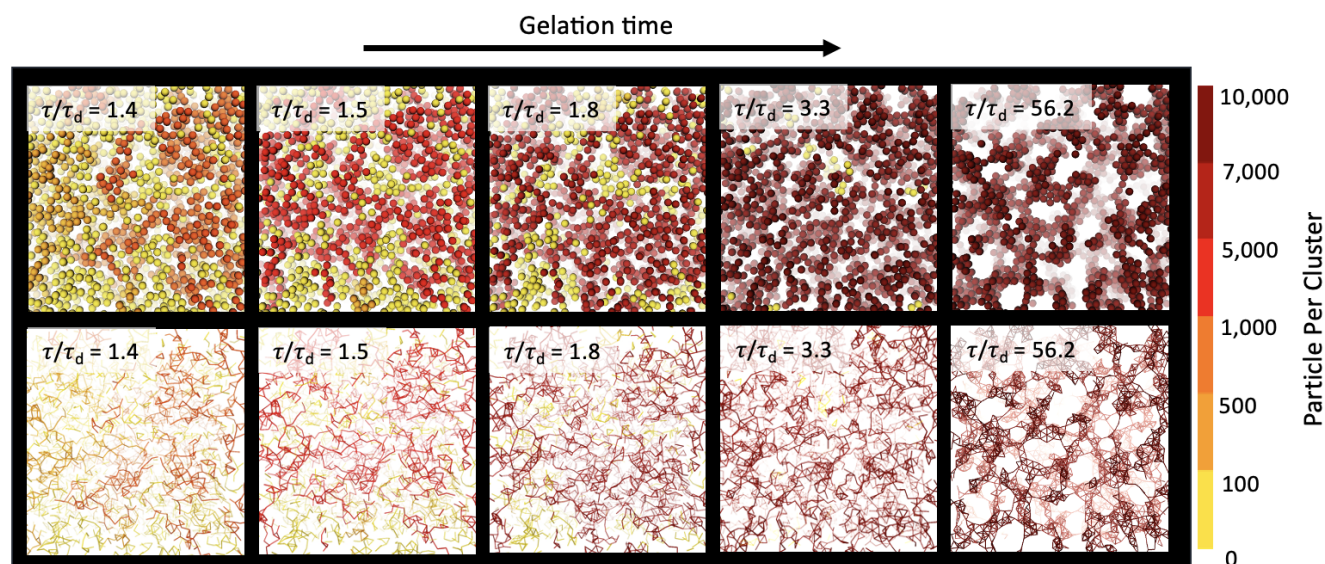
Figure 2. Snapshots of a colloidal system with a volume fraction of \phi = 0.20 and an attraction strength of U_0 = 20k_B T undergoing gelation at dimensionless times ( \tau/\tau_d ) 1.4, 1.5, 1.8, 3.3, 56.2 from left to right, where \tau_d is the diffusion time. ( Top row ): Colloidal assemblies, and ( Bottom row ): their resulting bonded structures over time. All colloids and their bonds are color-coded with respect to the number of particles within the clusters, provided in the scale bar. The process begins with the absence of large clusters in the initial stage and progresses to the largest cluster spanning the entire system, and ends with the coarsening of the particulate network.
