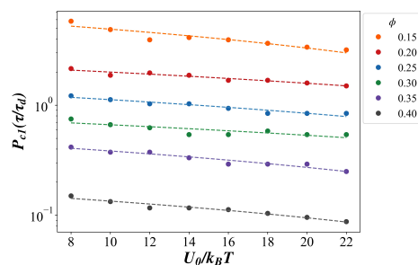
Figure 6. The percolation time, P_{c1} , for different volume fractions and attraction strengths.
