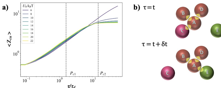
Figure 7. (a) Cumulative unique neighbors, Z_{cu} , of particles during gelation for \phi = 0.20 and different attraction strengths. Both transition points, P_{c1} and P_{c2} , are marked using vertical lines. (b) Schematic view of changes in Z_{cu} , in upper image at time t , with Z_{cu}^A = Z^A = 3 , and at time t + \delta t with Z_{cu}^A = 4 and Z^A = 3 .
