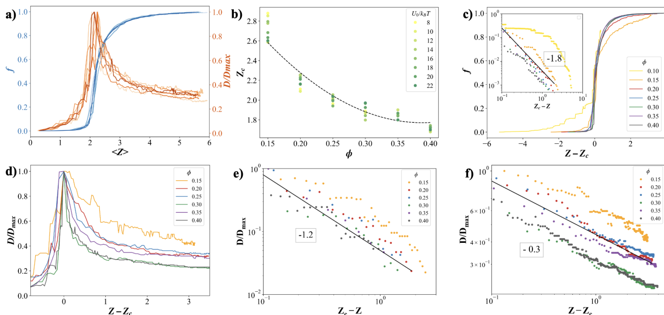
Figure 5. (a) Normalized network diameter (by its maximum value) and the fraction of particles within the largest connected components versus the ensemble-averaged coordination number, \langle Z \rangle , for all attraction strengths at \phi = 0.2 . (b) Critical coordination number, Z_c , for different attraction strengths and volume fractions. (c) Fraction of particles within the largest connected component, f , versus the re-scaled coordination number for all volume fractions at the attraction strength of U_0 = 20k_B T . The insert figure shows the same data in a power-law plot, characterized by an exponent of -1.8 . (d-f) The diameter of the largest cluster as a function of the re-scaled coordination number, featuring an exponent of -1.2 before (e), and -0.3 after (f) the critical point for all volume fractions.
