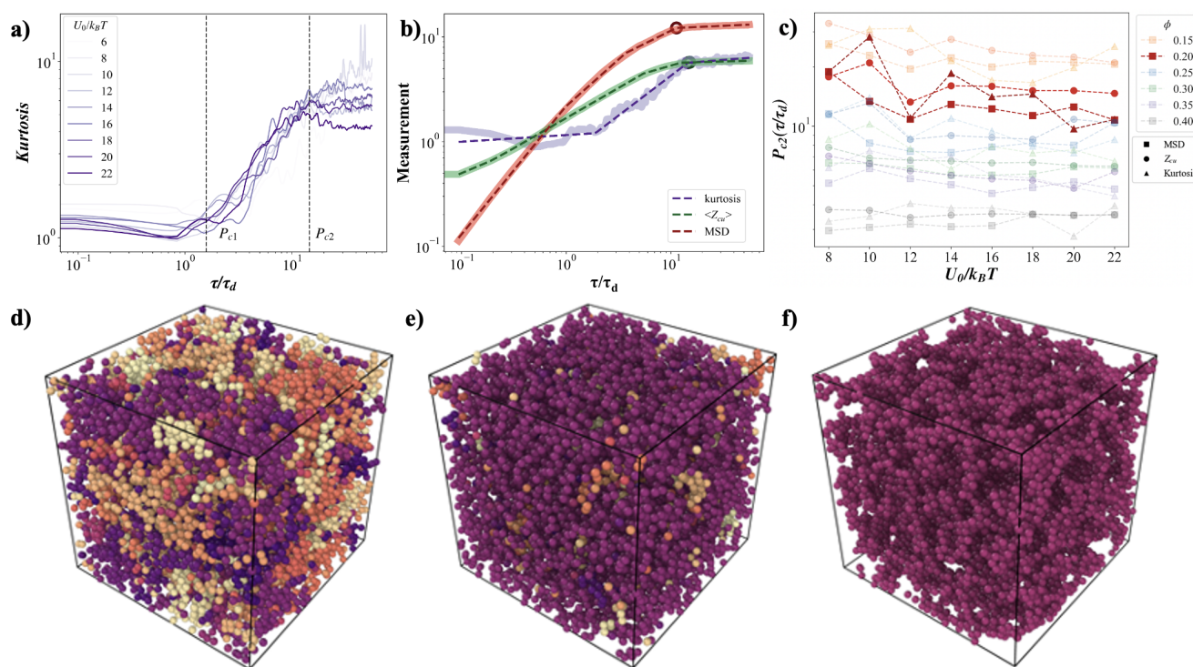
Figure 10. (a) Kurtosis of the Voronoi volume distribution versus time for various attraction strengths for the system with \phi = 0.2 . (b) Comparison of the second transition point across different measurements: mean square displacement (MSD), kurtosis, and unique neighbors ( Z_{cu} ) for a system with volume fraction \phi = 0.2 and attraction strength U_0 = 20k_B T . The plots are analyzed using linear regression, indicated by dashed lines. The point of slope change is marked as the second transition point. (c) The second critical point measured from Z_{cu} (circles), MSD (squares), and kurtosis (triangles) for \phi \geq 0.15 and all attraction strengths. Snapshots of the system with \phi = 0.2 and U_0 = 20k_B T : (d) before percolation, (e) at the percolation point, and (f) at the second transition point and end of coarsening. colors indicate particles belonging to the same cluster.
