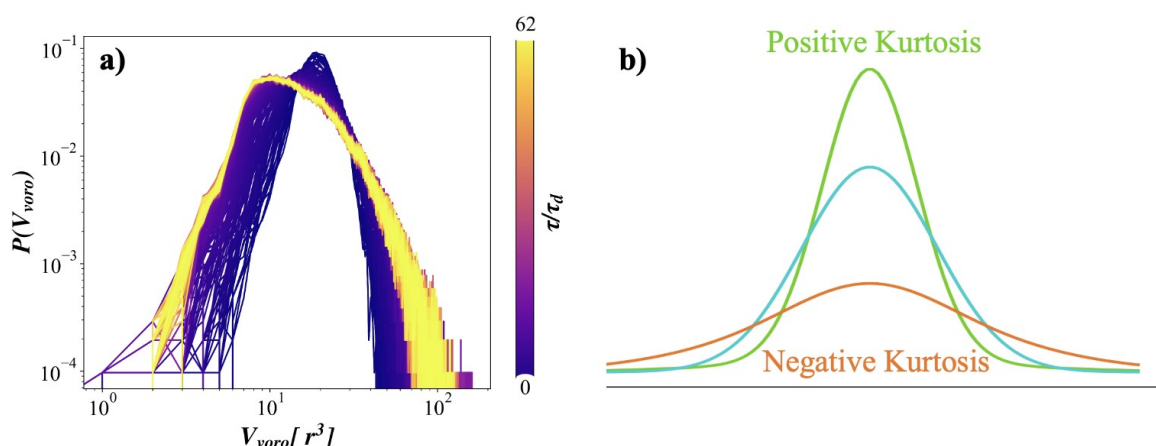
Figure 9. (a) Voronoi volume distribution at different times during the gelation process of a system with \phi = 0.2 and U_0 = 20k_B T . (b) schematic depiction of kurtosis, showing variations in data distribution at the peak and tails.
