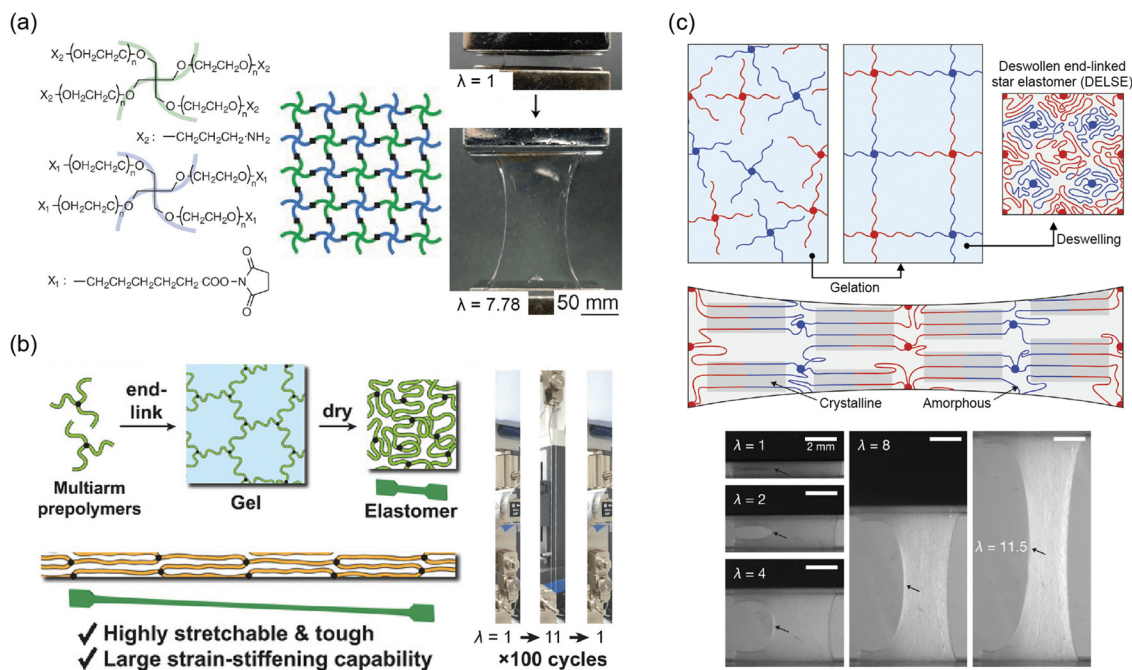
Fig. 8 Ideal network. (a) Tetra-armed hydrogels, with a well-organized network structure, increase fracture energy without compromising elasticity, maintaining mechanical integrity under repetitive loading. Reproduced with permission from ref. 141. Copyright 2014, AAAS. (b) Elastomer with a highly homogeneous network structure demonstrates both elasticity and notch resistance due to uniform stress distribution. Reproduced with permission from ref. 139. Copyright 2023, Wiley-VCH. (c) An ideal polyethylene glycol (PEG) network with a hierarchical structure of crystalline and amorphous phases shows high toughness and elasticity, attributed to the orderly arrangement of the polymer network. Reproduced with permission from ref. 138. Copyright 2023, AAAS.
