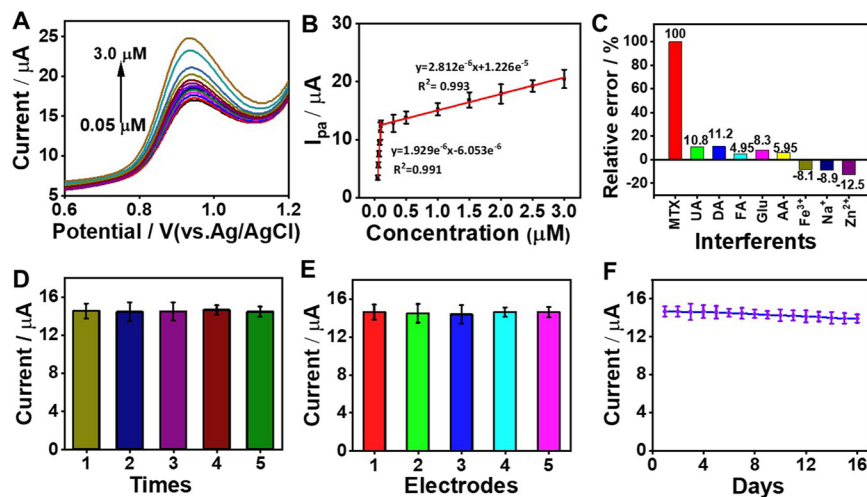
Fig. 6 (A) DPV curves of NiMn 2 O 4 /CNT-GCE recorded at various MTX concentrations ranging from 0.05 to 3.0 \mu M in 0.1 M PBS (pH 7.0). (B) Calibration plot showing the relationship between MTX concentration and I_{pa} . (C) Relative responses of the NiMn 2 O 4 /CNT-GCE to various interfering species (50 \mu M each) added to a 1 \mu M MTX solution in 0.1 M PBS (pH 7.0), normalized to the MTX response (1 \mu M MTX without any added interferents, set to 100%). (D) Repeatability of the sensor response to 1 \mu M MTX, evaluated using five consecutive measurements with a single electrode. (E) Reproducibility of the sensor response to 1 \mu M MTX, evaluated using five independently fabricated electrodes. (F) Long-term stability of the sensor monitored over 16 days with the electrode stored at 4 ^{\circ} C in 0.1 M PBS (pH 7.0).
