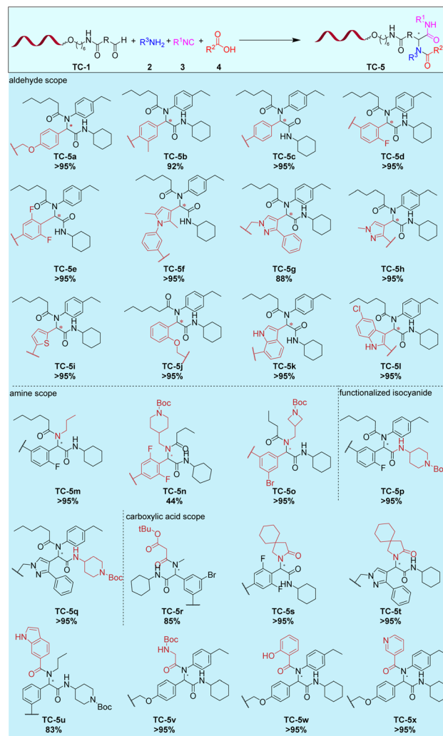
Fig. 3 Scope of the Ugi four-component reaction on 10mer TC-DNA. Reaction conditions: TC-1 (3 nmol) and copolymer (90 nmol) and primary amine 2 (6 \mu mol) in MeOH/CHCl 3 (50 \mu L; 3:1, v/v) for 3 h at rt. Addition of isocyanide 3 (6 \mu mol) and carboxylic acid 4 (6 \mu mol). The reaction was run for 16 h at 50 °C.
