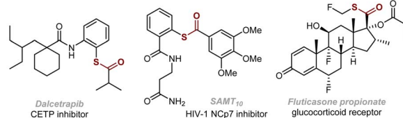
(b) Traditional methods for thioesters formation
