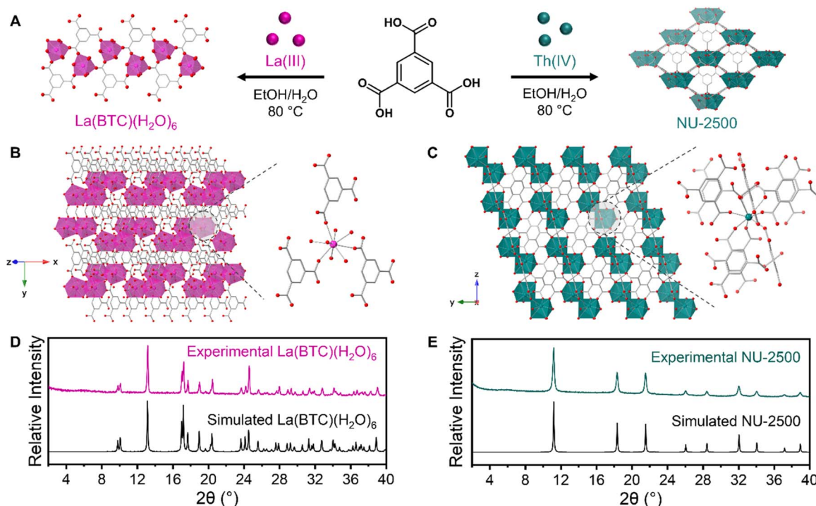
Fig. 2 (A) Scheme demonstrating crystallization of either [\text{La}(\text{BTC})(\text{H}_2\text{O})_6] or NU-2500 from 1,3,5-benzenetricarboxylic acid linker with \text{La}(\text{III}) or \text{Th}(\text{IV}) , respectively. Schematic representations of 3-D structures and individual metal ion nodes of (B) [\text{La}(\text{BTC})(\text{H}_2\text{O})_6] and (C) NU-2500. To account for the occupational disorder of BTC ligands within the NU-2500 crystal, this schematic is simplified to demonstrate average linker occupancy. Color code: La (magenta), Th (teal), C (gray), and O (red). Hydrogen atoms are omitted from the structures for clarity. Experimental PXRD patterns and simulated patterns from single crystal data for (D) [\text{La}(\text{BTC})(\text{H}_2\text{O})_6] and (E) NU-2500.
