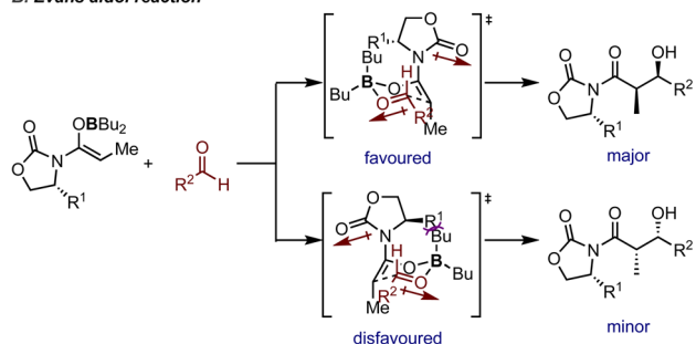
Fig. 2 A) Zimmerman–Traxler model (determination of relative configuration); B) an illustrative example for an Evans aldol reaction (absolute configuration controlled by the chiral auxiliary).
