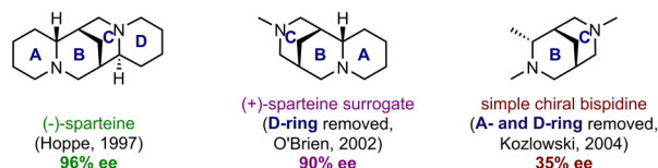
Fig. 3 (A) 3D structure of (–)-sparteine; (B) sparteine-mediated asymmetric lithiation and results with other diamines as comparisons.
