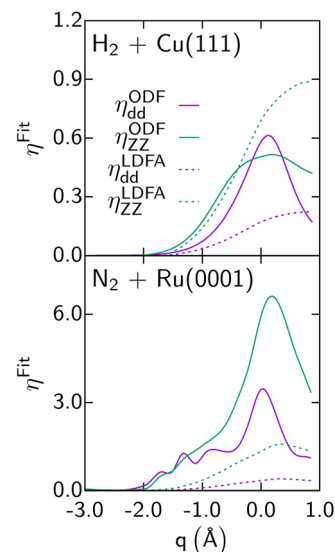
Fig. 11 Diagonal elements of the friction tensor, \eta_{\text{qq}} (in m eV ps Å -2 ), are shown as a function of q ( d is the bond distance of the molecule, Z the distance of the molecule's center of mass to the surface) for the LDFA and the ODF approximations, as computed for H 2 + Cu(111) 146 and N 2 + Ru(0001). 69 Data taken from ref. 146 and 69. This figure has been reproduced from ref. 13 with permission from the Royal Society of Chemistry, copyright 2021.
