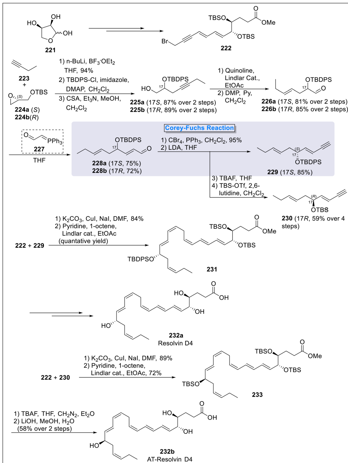
Scheme 22 Total synthesis of resolin D4 232a and its 17( R )-hydroxy-epimer 232b by Nshimiyimana and coworkers.
