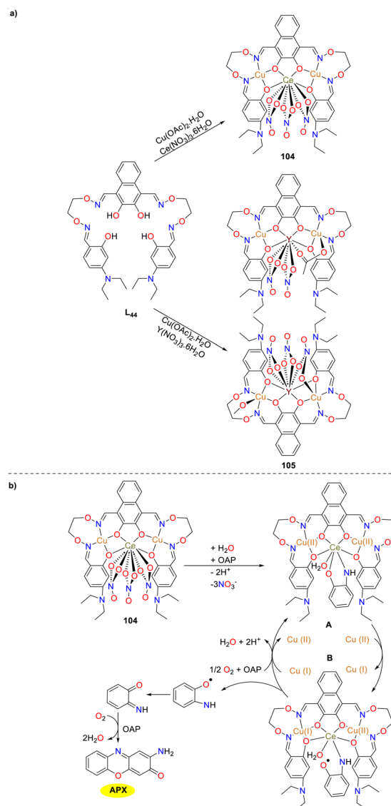
Scheme 41 Synthesis of complexes 104 and 105 and the proposed oxidation mechanism (ref. 66).
