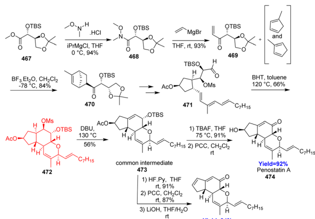
Scheme 61 Total synthesis of penostatin A ( 474 ) and C ( 475 ). 125
