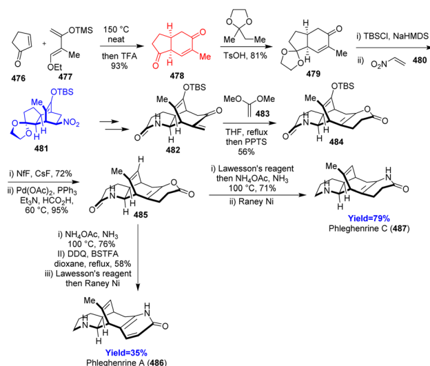
Scheme 62 Total syntheses of phlegghenrines A ( 486 ) and C ( 487 ). 126
