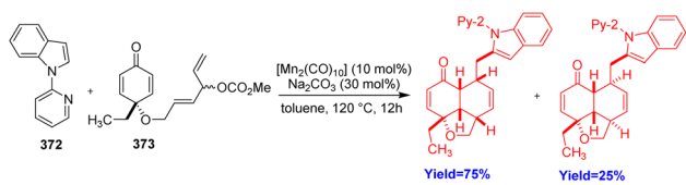
Scheme 47 Synthesis of 6/6/5-fused tricyclic terpenoid scaffold. 101
