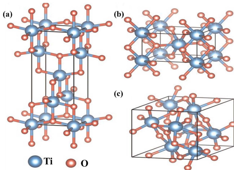
Fig. 5 Typical ball-stick crystal structure of \text{TiO}_2 polymorphs. (a) Anatase (tetragonal), (b) rutile (tetragonal), and (c) brookite (orthorhombic). 54
