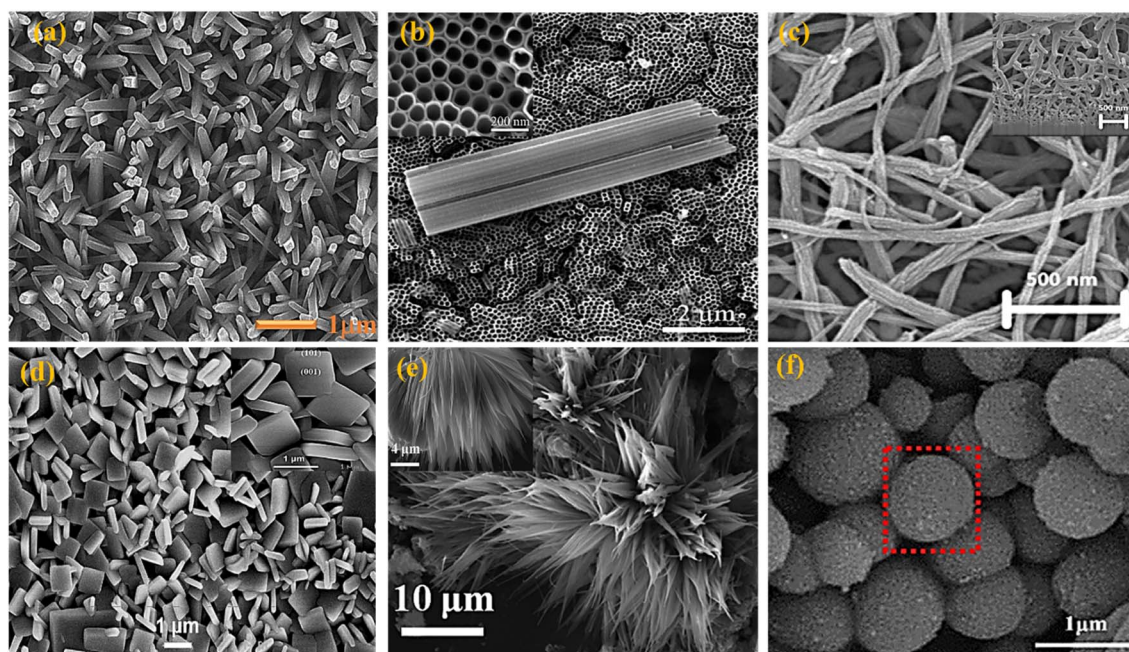
Fig. 6 FESEM images of various \text{TiO}_2 photoanodes including 1D, 2D and 3D structures explored for DSSC application. (a) Nanorods, 58 (b) nanotubes, 57 (c) nanowires, 58 (d) nanosheets, 59 (e) nanoflower, 60 and (f) nanosphere. 61
