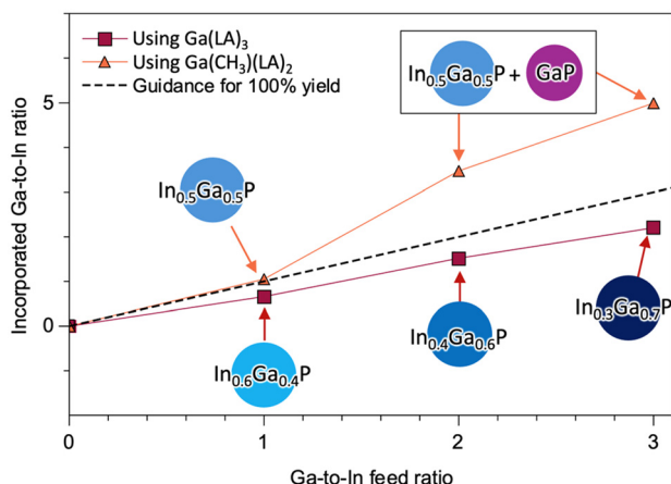
Fig. 3 Incorporated Ga-to-In ratio in \text{In}_{1-x}\text{Ga}_x\text{P} QDs characterized using ICP-OES. The \text{In}_{1-x}\text{Ga}_x\text{P} QDs were synthesized with varying Ga-to-In feed ratios of 1, 2, and 3, using \text{Ga}(\text{LA})_3 (red squares) and \text{Ga}(\text{CH}_3)(\text{LA})_2 (orange triangles). The dashed line serves as a guide representing unity reaction yield.
