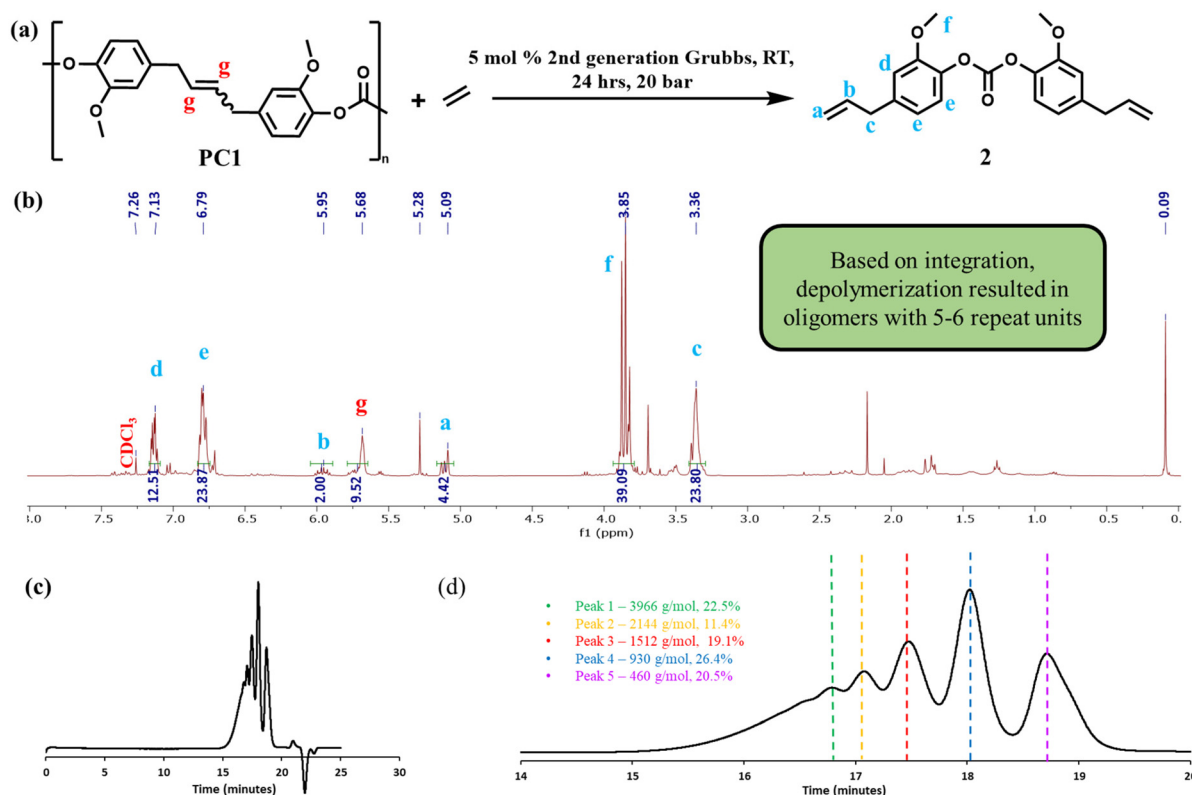
Fig. 5 (a) Ethenolysis scheme for depolymerization of polycarbonates. (b) ^1\text{H} NMR spectrum of depolymerized PC1 low in \text{CDCl}_3 . (c) GPC chromatogram of ethenolysis products derived from PC1 low . (d) Magnified view of the GPC chromatogram of depolymerized PC1 low .
