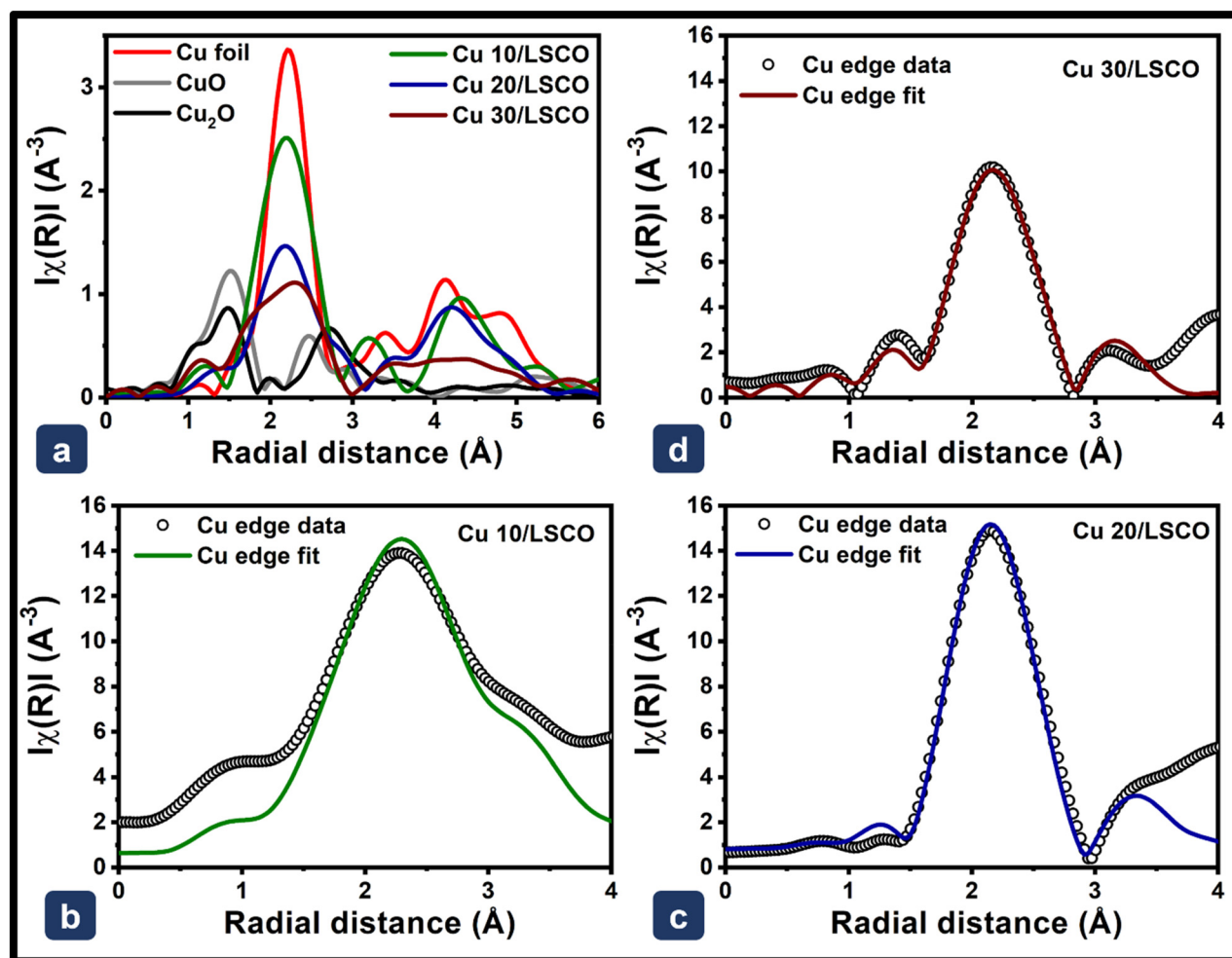
Fig. 3 (a) Fourier-transformed Cu K-edge EXAFS spectra of Cu x /LSCO samples ( x = 10%, 20%, and 30%) compared with the reference spectra of Cu foil, CuO, and \text{Cu}_2\text{O} . (b–d) Fourier-transformed Cu K-edge EXAFS data (scatter points) and the corresponding fitting curves (solid lines) for (b) Cu 10/LSCO, (c) Cu 20/LSCO, and (d) Cu 30/LSCO.
