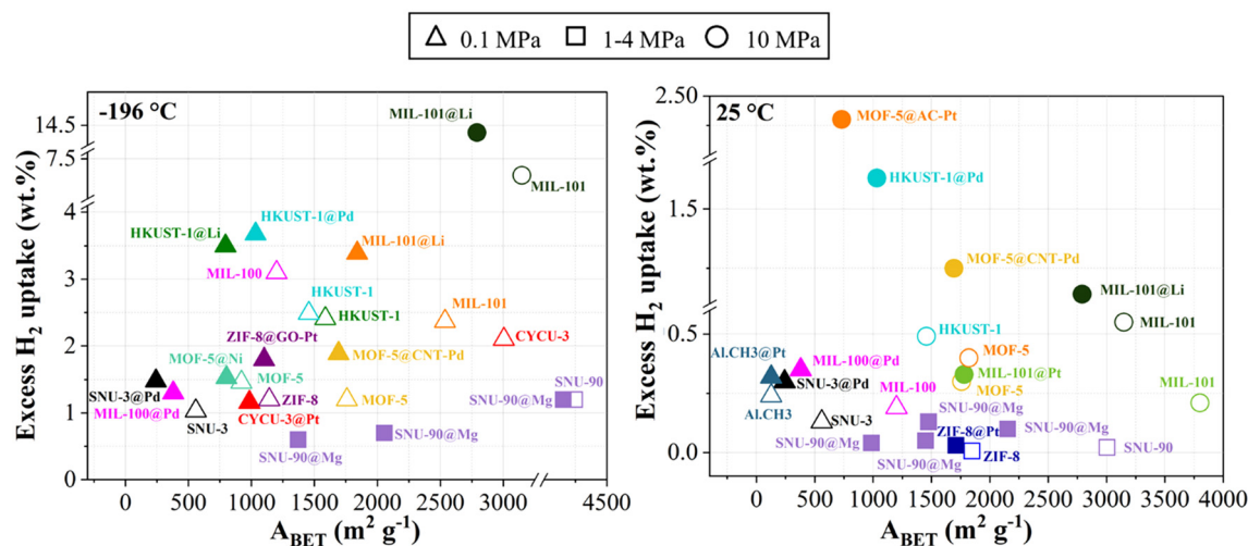
Fig. 8 Influence of adding metal particles into MOFs on the H 2 storage capacities of the resultant hybrid materials ( \bullet \circ ref. 204); ( \triangle , \square , \circ ref. 205); ( \triangle , \square ref. 206); ( \triangle , \square , \circ ref. 207); ( \bullet , \circ , \triangle ref. 90); ( \square , \bullet ref. 208); ( \bullet , \triangle , \square ref. 209); ( \triangle , \square ref. 210); ( \bullet , \triangle ref. 162); ( \bullet , \circ ref. 211); ( \square , \bullet ref. 212); ( \triangle , \bullet ref. 213); ( \triangle , \square ref. 214).
