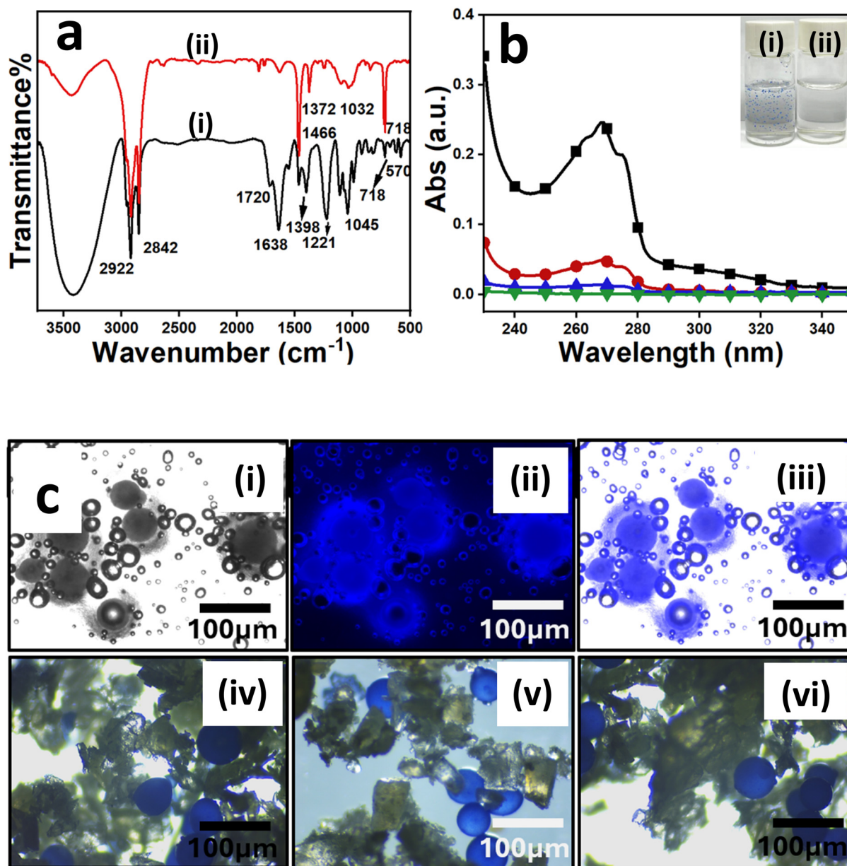
Fig. 11 FTIR spectra (a) of the facial scrubber (i) and blue beads found in the scrubber (ii). UV-Vis spectra (b) of the facial scrubber before (i) and after extraction by PA1 (ii), PA2 (iii), PA3 (iv). The inset image in (b) indicates the solution of the commercial scrubber before (i) and after (ii) extraction. Optical fluorescence images (c) of polypropylene beads found in a commercial facial scrubber in different modes, such as DIC (i), DAPI (ii), and merged (iii) view of the particles. The air bubbles are seen as circles in the solution. Stereomicroscopic images of the PA1 (iv), PA2 (v), and PA3 (vi) polymers after adsorption of the facial scrubber.
