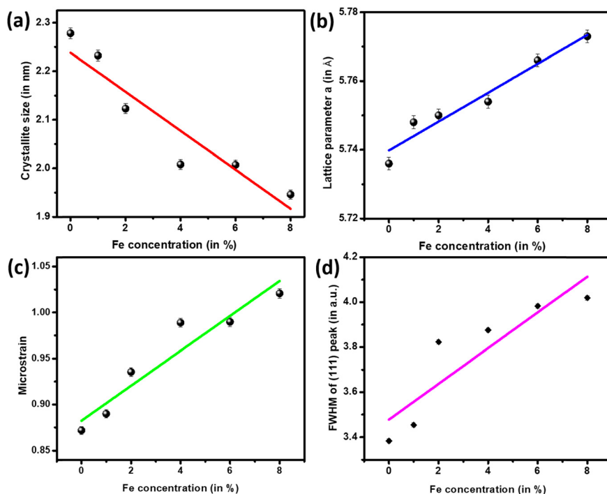
Fig. 2 (a) Average crystallite size variation, (b) variation in lattice parameter ' a ', (c) variation in micro-strain, (d) variation in FWHM of peak (111) with varying Fe doping concentration in CdS QDs. The crystallite size is decreasing with increasing doping concentration owing to quantum confinement.
